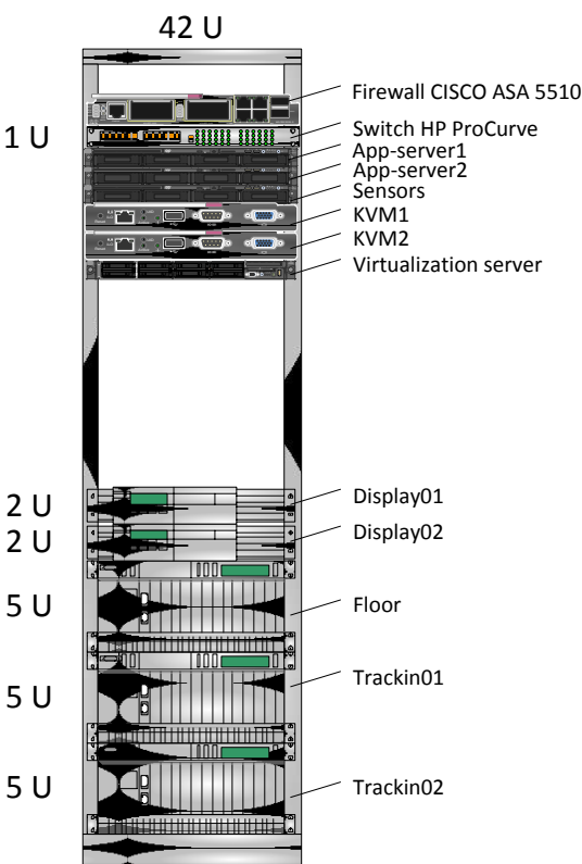
Fig. 10 - Final configuration of XIM 2.0 rack after upgrade
