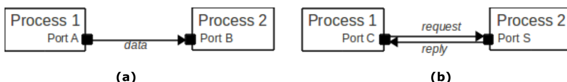
Figure 2: (a) The publisher/subscriber interaction mode between port A (publisher) and B (subscriber) of processes 1 and 2. (b) Client / server interaction mode between ports C (client) and S (server). First the client sends a request, and once the requested computations have been performed on the server it sends a reply back to the client.
