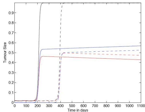
Figure 7.3 Simulation of tumour evasion from immune control in a purely temporal setting (spatial aspects disregarded). Solid lines N=4, dashed lines N=10.
