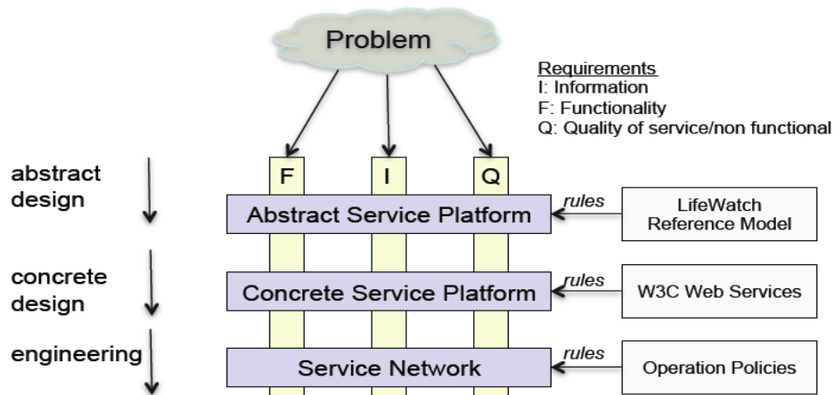
Figure 10: Abstract and concrete service platforms
