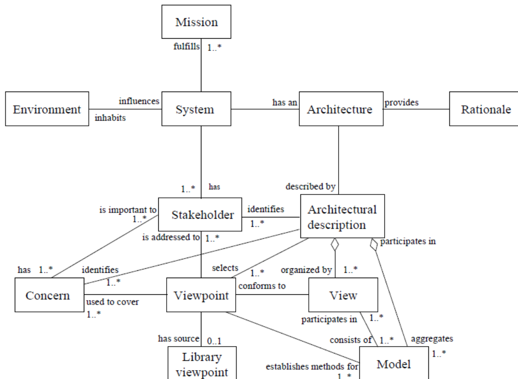
Figure 1: Conceptual model of architectural description from IEEE1471.
