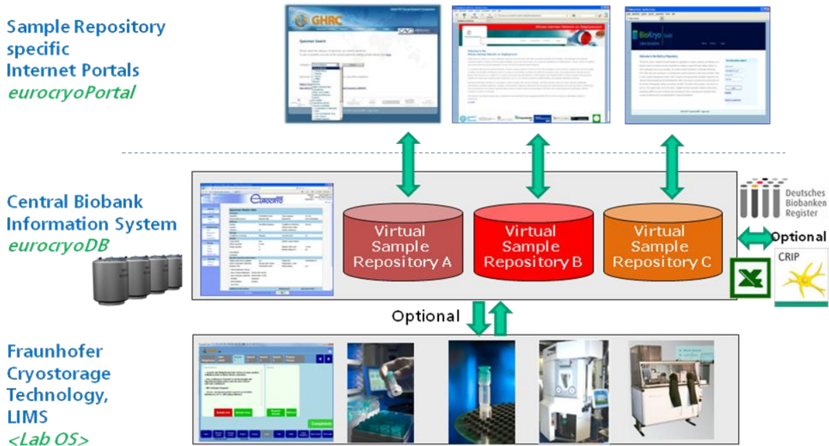
Figure 30: Overview of the eurocryoDB biomaterial management platform.
