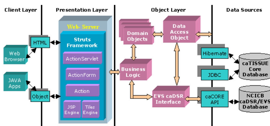
Figure 2: caTissue Architecture 22 .
