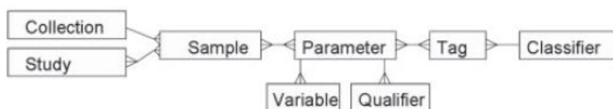
Figure 20: High level data structure in SAIL according to Gostev et al.
