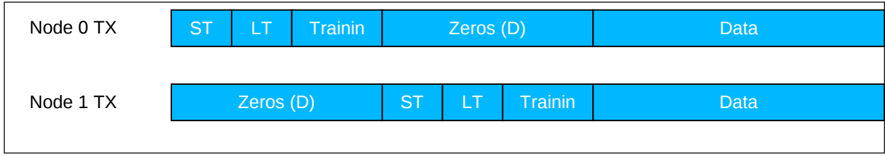
Figure 56. Time domain representation of the full-duplex frame.
