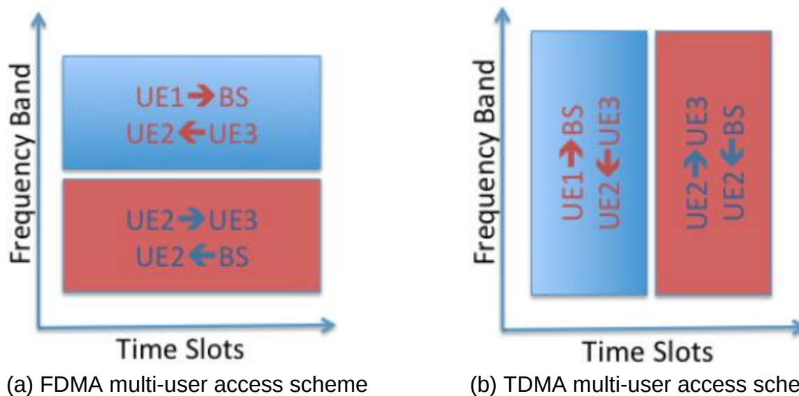
Figure 14. Full-duplex device-to-device communications: user scheduling and resource allocation method 2.
