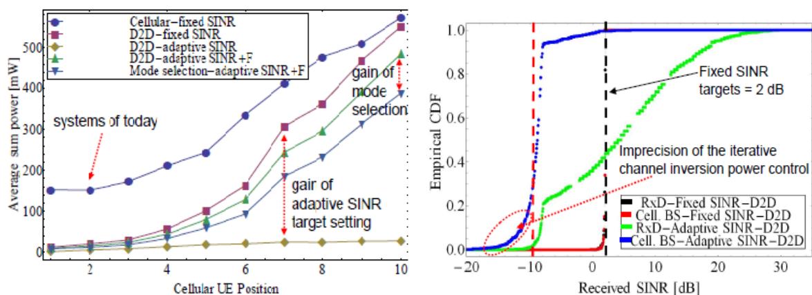
Figure 2-3. Comparisons of the average sum power and the received SINR.
