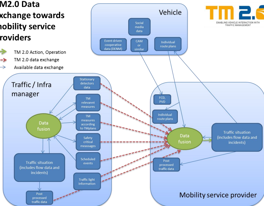
Figure 3: TM2.0 data exchange towards mobility service providers
