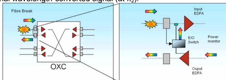
Figure 46 - Scheme of the stabilization technique based on channel replacement
