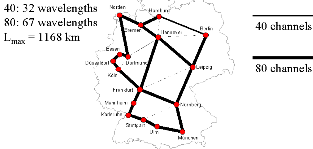
Figure 38 - Topology for the 2006 scenario with 10% of the wavelengths free
