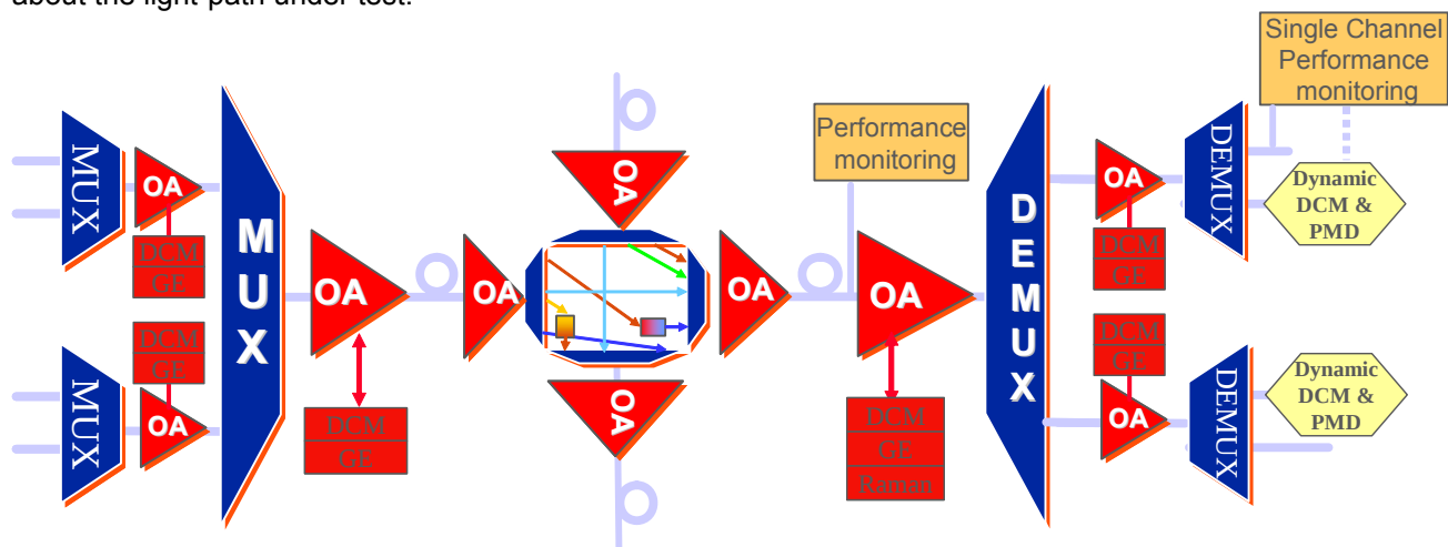
Figure 34 - Transmission system with optical monitoring and adaptive compensators
