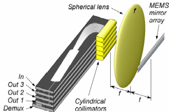
Figure 55 - WSS from Lucent [ECOC2005 Th3.6.4]
