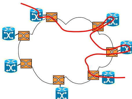
Figure 8 - the OTN receive the traffic from the IP network (i.e. from routers) and their role is only to groom IP traffic with circuit native, but the switching is provided at IP layer. A second role of the OTN is to provide a more cost-effective and fast restoration
