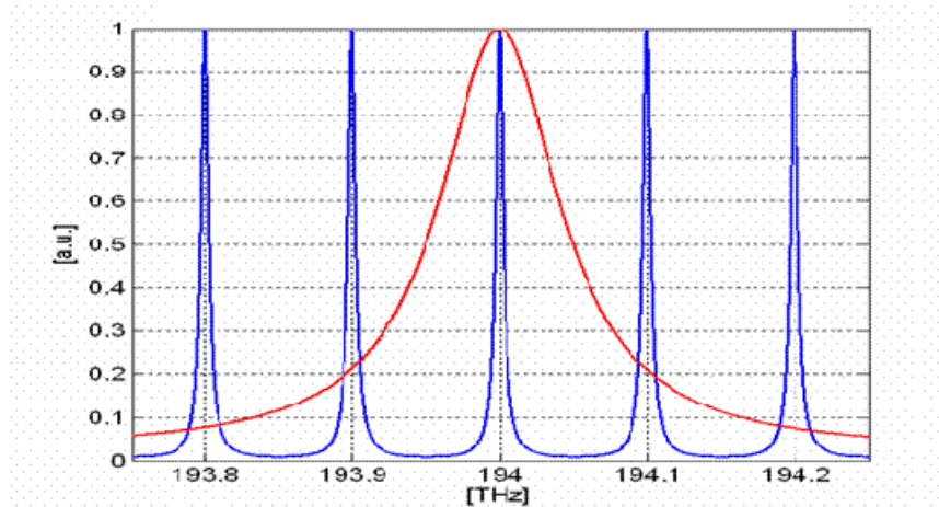
Figure 53 - ECL laser: The blue line (narrow spectra) is the spectral response of the cavity etalon, the red one (broad spectrum) is the tuneable mirror transfer function selecting one channel
