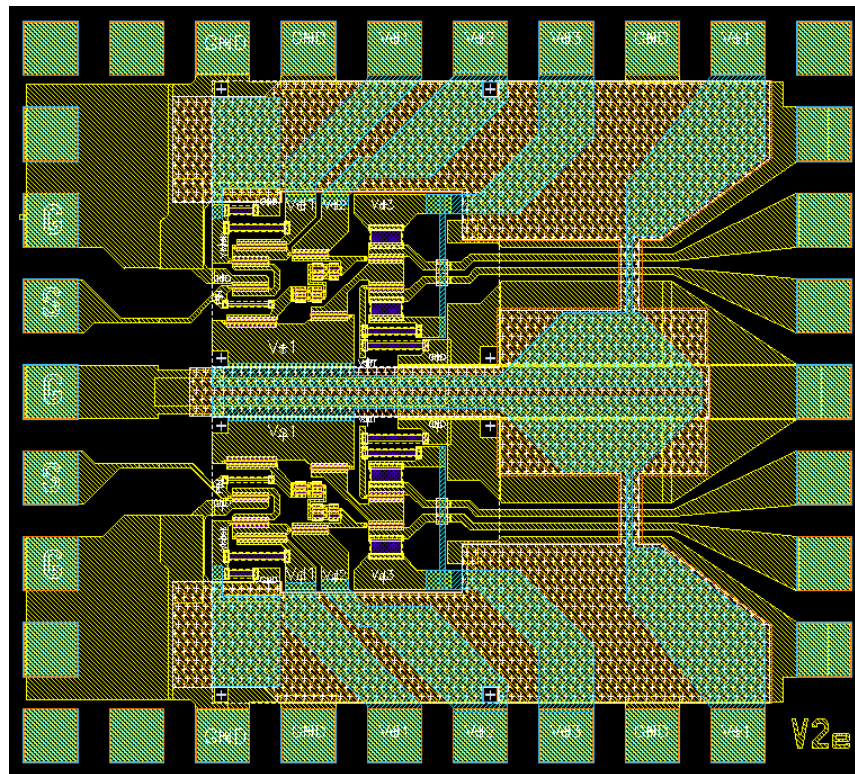
Fig. 30: EE-TIA for testing the TIA without pin-diodes
