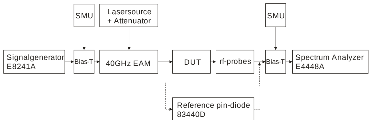
Fig. 43: Schematic diagram of the developed optical/electrical on-wafer measurement setup
