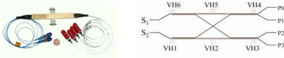
Fig. 41: CeLight's optical 90^\circ hybrid CL-QOH-90 (left) and its schematic (right).
