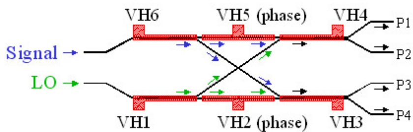
Fig. 7: Connection scheme of the 90° optical hybrid
