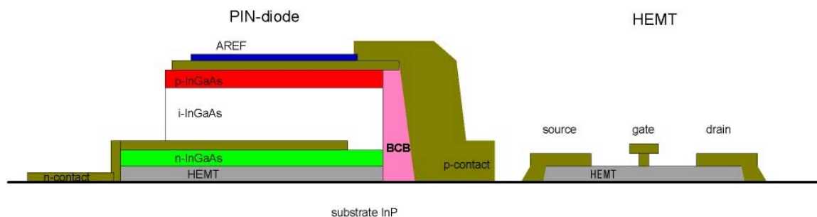
Fig. 21: Cross section of the proposed integration of pin-diode and HEMT for the balanced photoreceiver.
