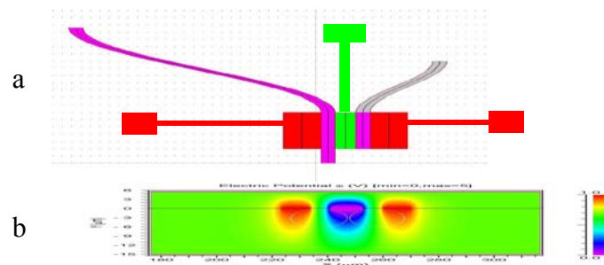
Fig. 5: a) the waveguides and the electrodes layout. The pink waveguide is the input (left). The red electrodes are for DC bias. The green electrode (middle) is the ground. b) The electrostatic field distribution in the coupler cross section.
