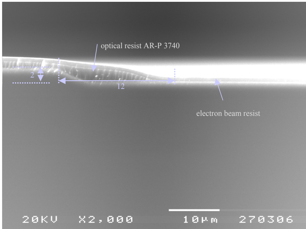
Fig. 25: SEM image of photo resist on 2\text{ }\mu\text{m} mesa structure
