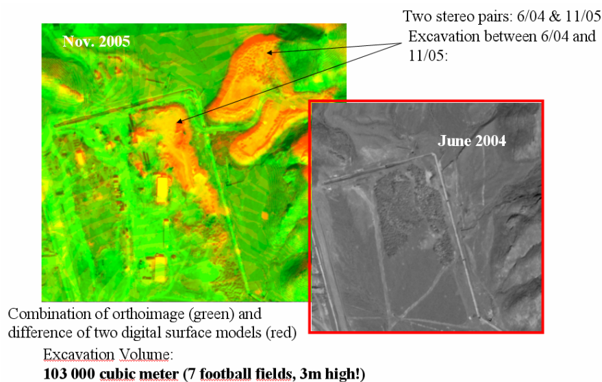
Subsurface constructions, underground activities at Esfahan. 3D change detection using stereo pairs of June 2004 and November 2005 © DLR
