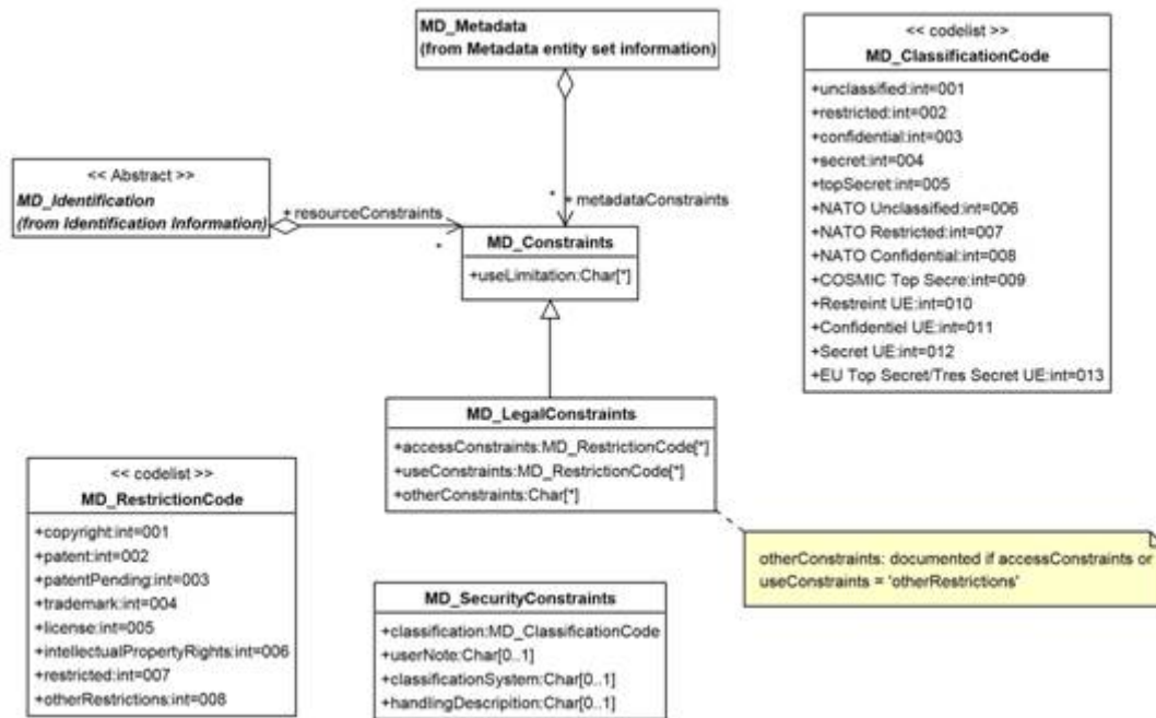
Example UML Diagram for the 'Constraint' Metadata Elements
