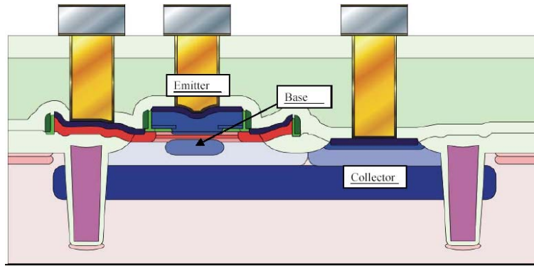
Fig. 28: HBT integration in the CDR1 BiCMOS technology
