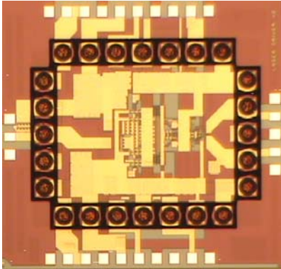
Fig. 30: Laser diode driver ICs with Cu (left) and SnPb bumps (right)
