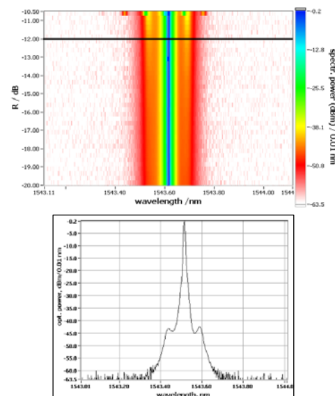
(c) Optical feedback measurements indicating feedback threshold of the CSDFB device to be higher by 4-5 dB as compared to a BH-DFB laser with traditional design. Measurements were made in accordance with IEEE Standard 802.3ae™-2002.
