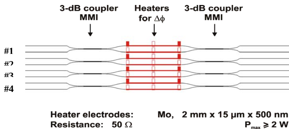
Fig. 17: Schematic layout of thermo-optically controlled MZIs functioning as VOAs. Only one heater stripe will be activated to detune the MZI, whereas the other one is available for redundancy reasons.
