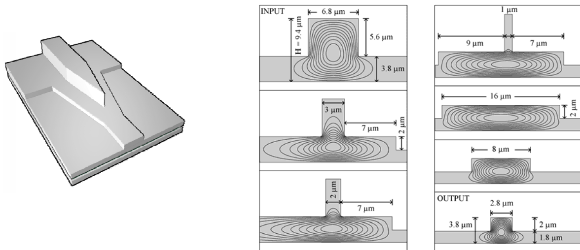
Fig. 6: Schematic view of a vertical taper fabricated with multi-step patterning. Note that in reality the taper is much longer. Input (e.g. from fiber) at the top side, output into chip waveguide: bottom side ( left ). Different cross-sections along the vertical taper with calculated intensity distributions for the fundamental TE mode. The results for TM polarisation are almost identical. Misalignment of 1 \mu\text{m} is assumed between the two masks. Otherwise dimensions are identical to those measured from the fabricated devices in 9 \mu\text{m} SOI ( right )
