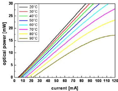
(a) Temperature dependent P-I curves 20°C slope efficiency: 0.38 W/A; etched AR coated front facet; backside as-cleaved
