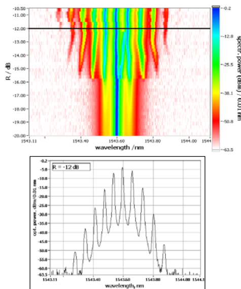
(c) Optical feedback measurements indicating feedback threshold of the CSDFB device to be higher by 4-5 dB as compared to a BH-DFB laser with traditional design. Measurements were made in accordance with IEEE Standard 802.3ae™-2002.
