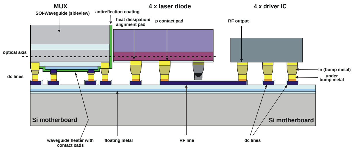
Fig. 3: Silicon optical bench (SiOB) based hybrid integration scheme.
