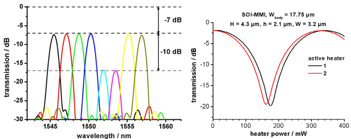
Fig. 18: Measured characteristics of an 8-channel 200 GHz AWG integrated with a MZI-VOAs; channels #5 and #6 are attenuated by 10 dB in this example. Maximum attenuation of > 15 dB is achieved at 170 mW of heater power (right)
