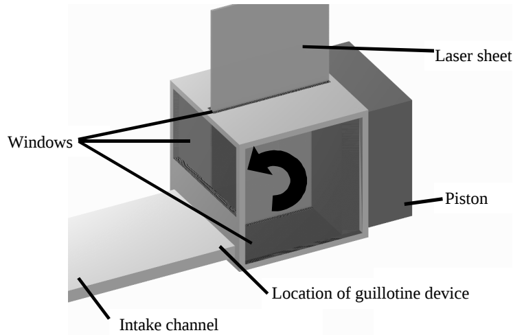
Figure 2-10: Sketch of the compressed tumble, square piston engine
