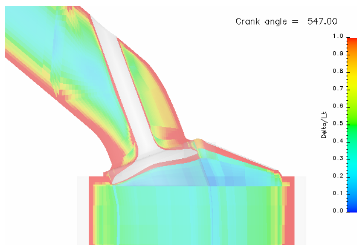
Figure 2-9: Estimation of the current mesh resolution for a typical engine using the ration of the filter width (grid size) and the integral length scale.
