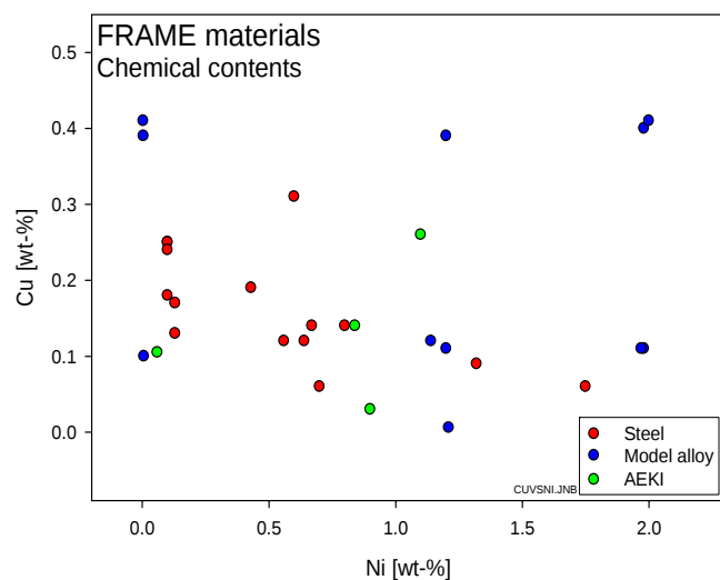
Figure 4. Copper and nickel contents of FRAME materials
