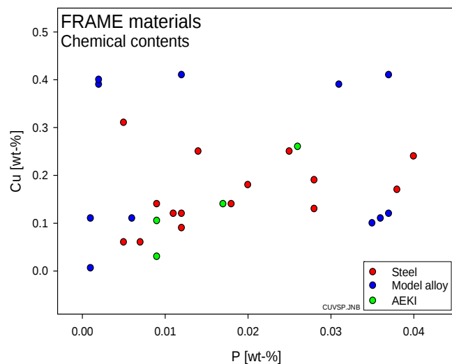
Figure 3. Copper and phosphorus contents of FRAME materials
