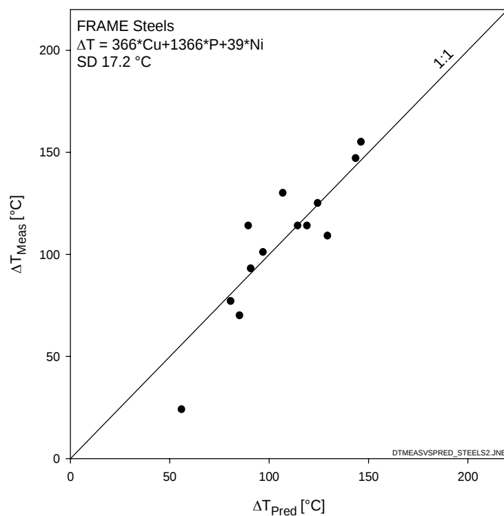
Figure 16. The best fit to steel data excluding the two high-nickel steels. The deviating low-shift point is FFA with Cu = 0.06 %, P = 0.005 % and N = 0.70 %, i.e. the general formula based on all data can not describe the nickel effect with absence of Cu and P
