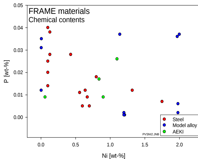
Figure 5. Nickel and phosphorus contents of FRAME materials
