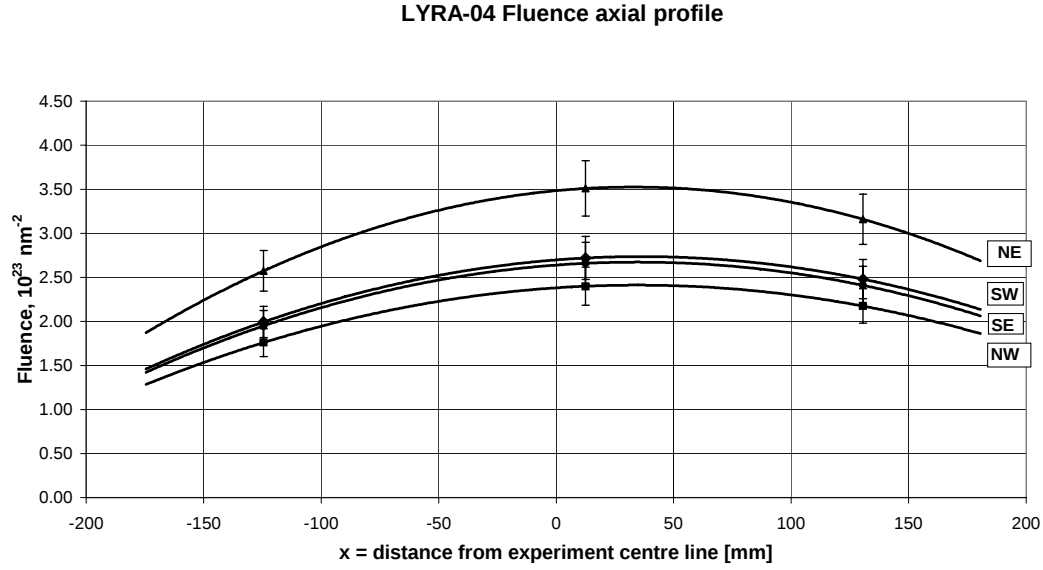
Figure 7. Vertical neutron fluence distribution along the four capsule corner lines NE, SW, SE and NW. The points with error bars identify the corner positions of the capsule (top, middle and bottom)
