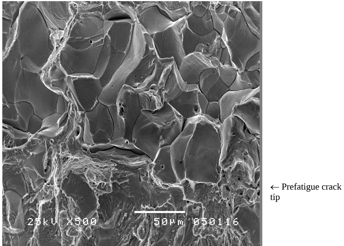
Figure 17. Model alloy 176, specimen C03, IG = 95 %, ductile 5 %, T = 331\text{ }^{\circ}\text{C} , K_{JC} = 75\text{MPa}\sqrt{\text{m}}
