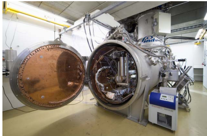
Figure 7: The HoBiCaT facility at BESSY has been used for many cavity tests.
