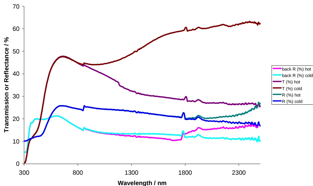
Figure 3. Transmission and reflectance data for a 1% tungsten doped \text{VO}_2 (m) film.
