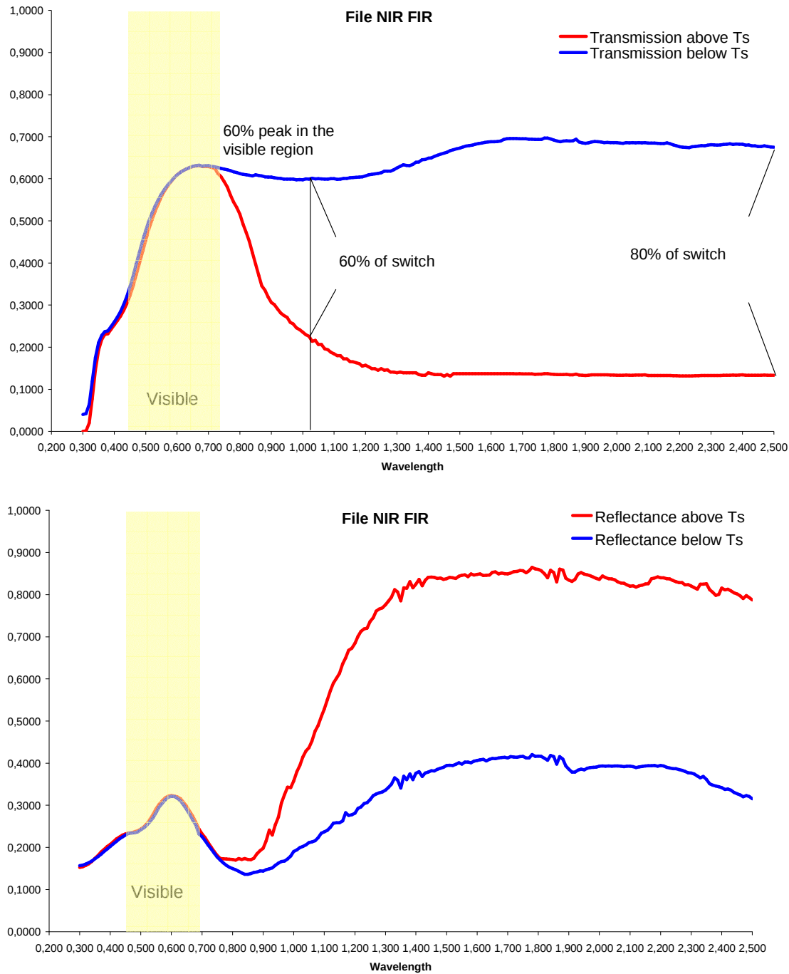
Figure 5: Ideal spectra (NIR-FIR) simulated to evaluate the energy performance in cooling dominated climates with respect to the benchmark (transmittance and reflectance)
