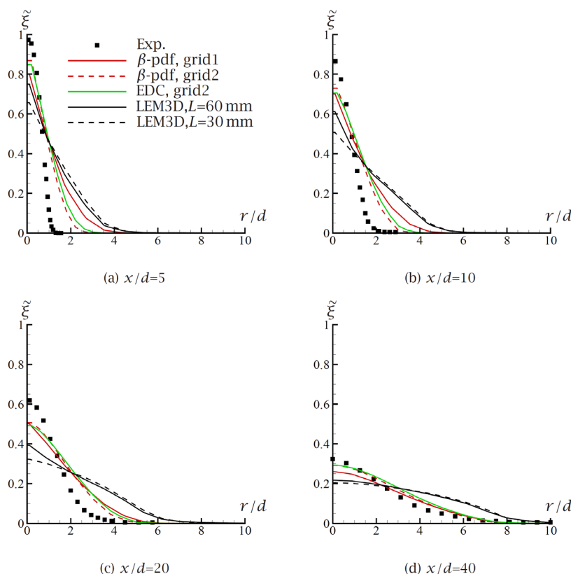
Figure 25: Radial mixture fraction profiles at 4 selected downstream positions in a non-premixed turbulent jet flame (DLR-A). Comparison with standard reaction-mixing models and experimental data from Meier et al. 2000
