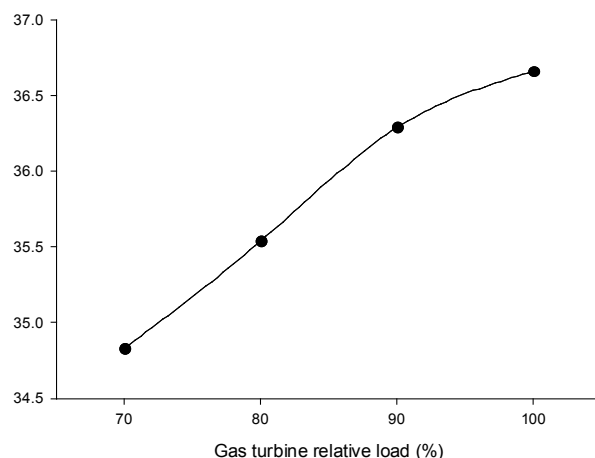
Figure 7 The net plant electrical efficiency as a function of gas turbine relative load
