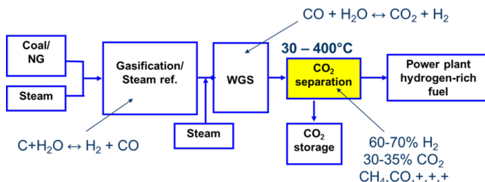
Figure 11 Positioning of CO 2 separation in the IGCC power plant
