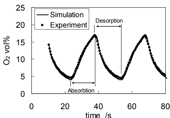
Figure 22 Oxygen content in the gas exiting a bed of LSCF perovskite wash-coated monoliths at 600^\circ C submitted to air – N_2 cycles
