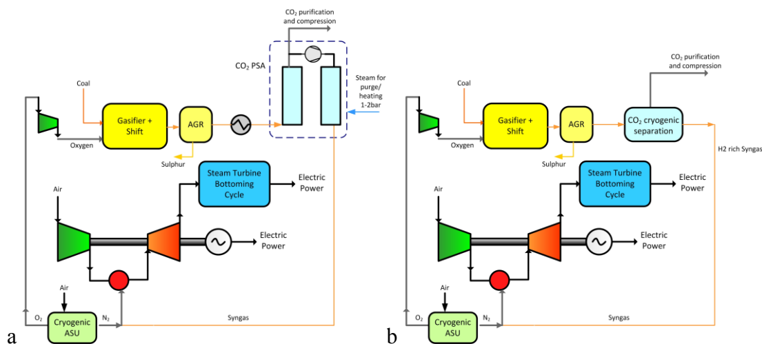
Figure 6 a) CO 2 separation with Pressure Swing Adsorption (PSA) b) CO 2 separation with Low Temperature (LT)
