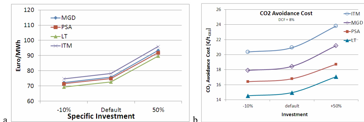
Figure 10 a) Cost of electricity versus specific Investment Figure 13. CO 2 avoidance cost in connection with the specific investment
