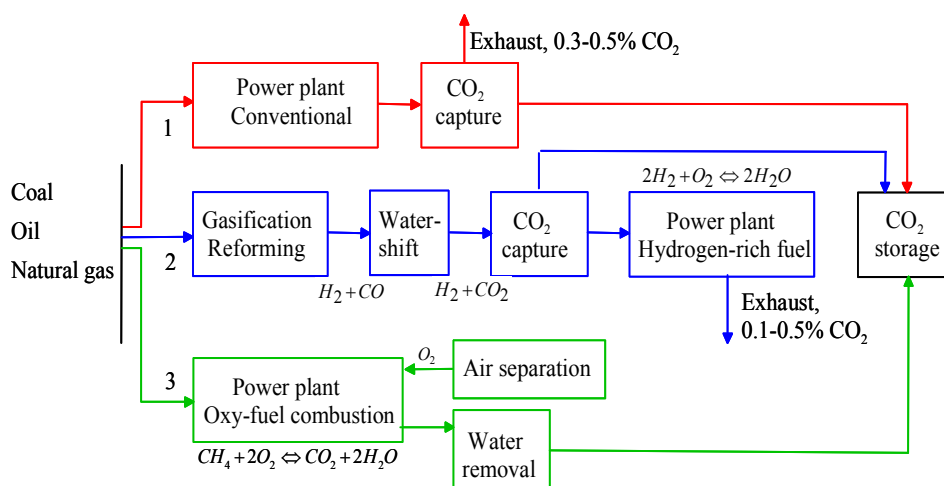
Figure 1 Capture routes for CCS
