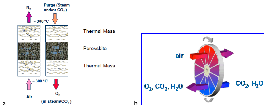
Figure 21 a) schematic of the CAR b) schematic of the rotating sorbent bed process
