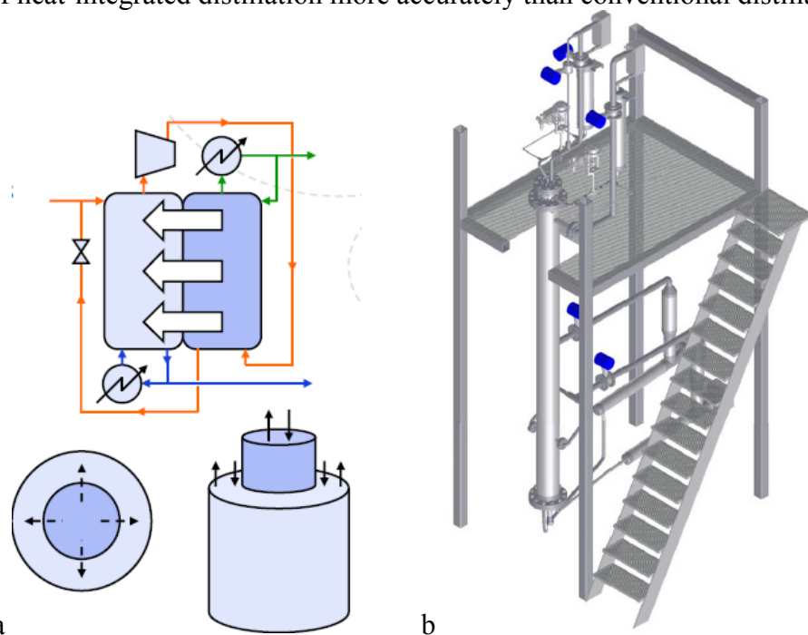
Figure 23 a) Concept of heat integrated distillation column (HIDiC) b) Experimental setup for the HIDiC, Pilot 3
