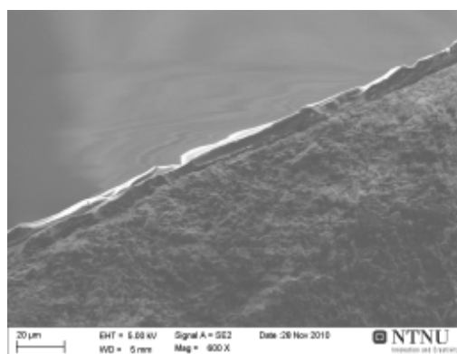
Figure 13 The SEM image of a carbon layer
