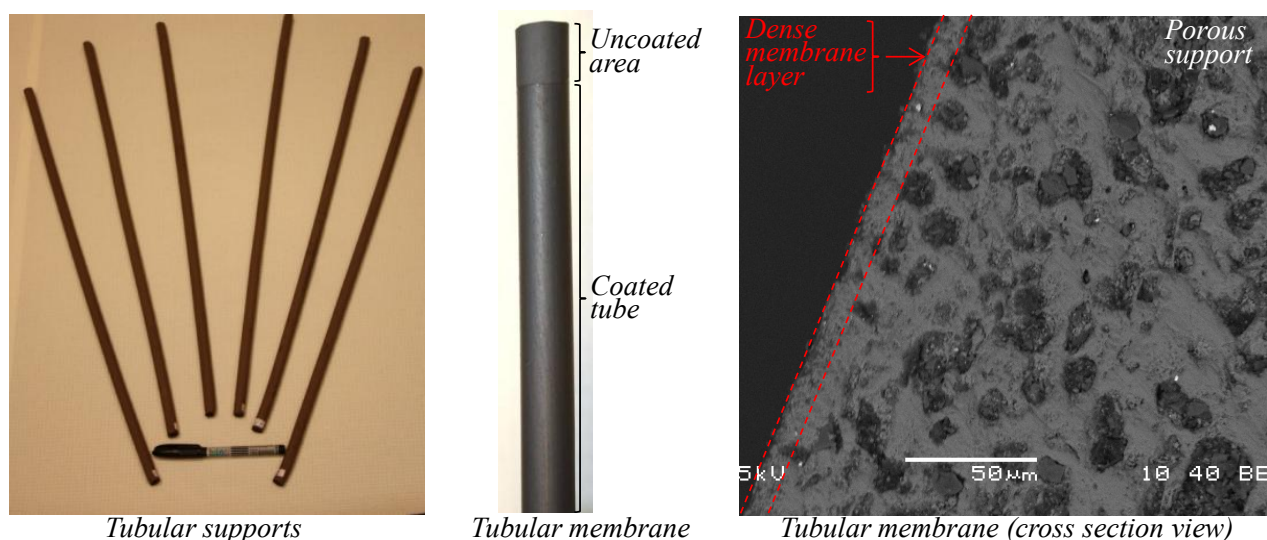
Figure 20 Examples of extruded tubular supports and membranes coated with thin dense layers
