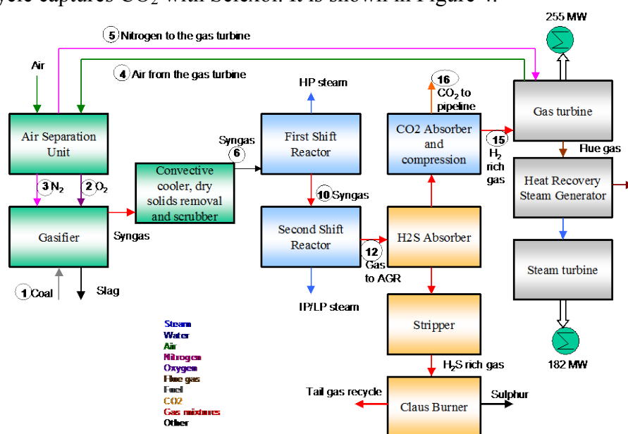
Figure 4 Base case - CO 2 capture with selexol (EBTF).
