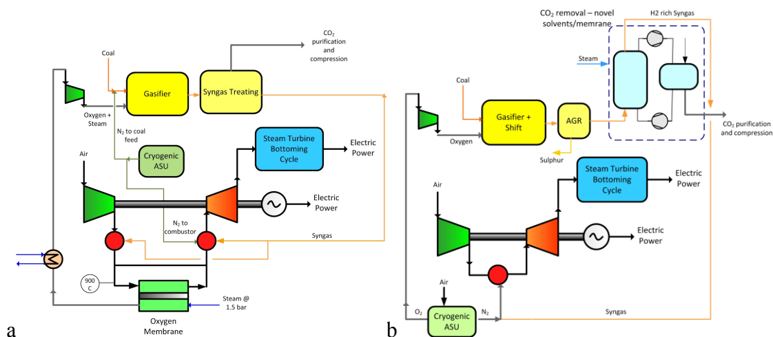
Figure 5 a) Air separation with Oxygen Transfer Membrane (OTM) b) CO 2 separation with solvent and Membrane Gas Desorption (MGD)
