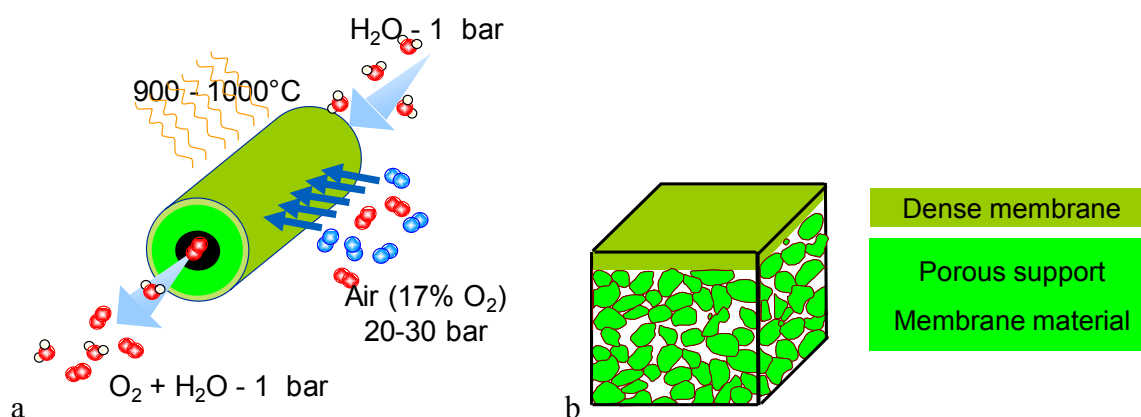
Figure 19 Concept of tubular OTM with operating conditions defined within DECARBit (a) and the asymmetric membrane architecture (b).
