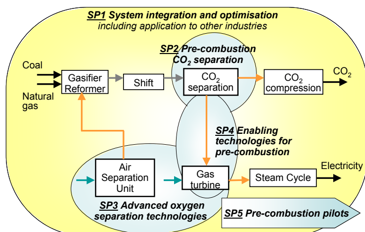
Figure 2 DECARBit Sub Project work focus in a generic pre-combustion plant
