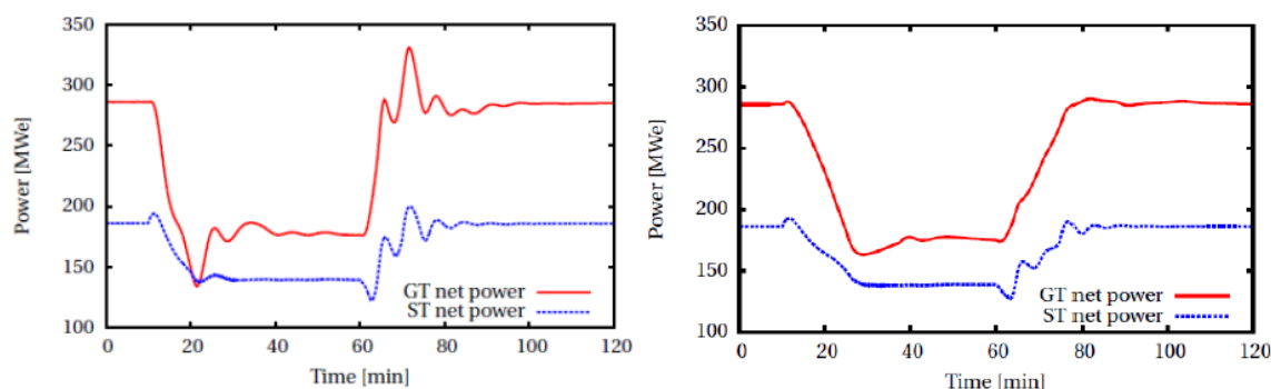
Figure 8 Gas turbine and steam turbine net power control, non-optimized versus optimized load variation procedure
