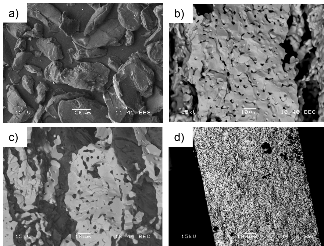
Figure 14 Fig.3 SEM micrographs of a) chitosan granules; cross-section views of b) CeO 2 porous disk before infiltration; c) and d) CeO 2 porous disk after infiltration in Li/K melt (Li 0.62 K 0.38 ) 2 CO 3 with two different magnifications
