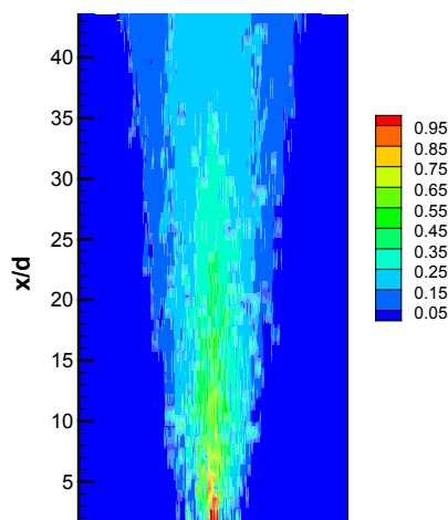
Figure 24 Snapshot of a LEM3D-RANS simulation. Contours of mixture fraction in the non-premixed turbulent jet flame DLR-A
