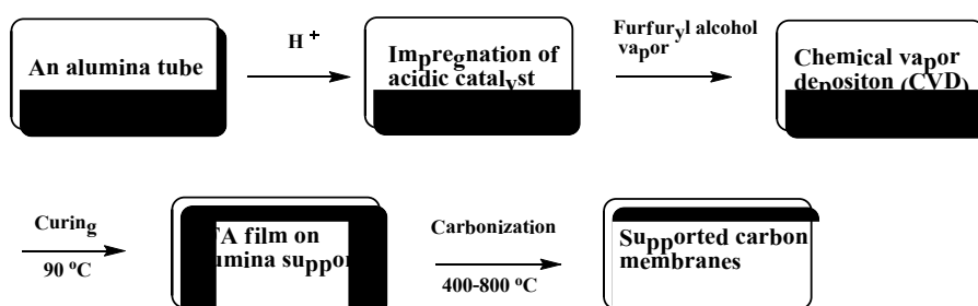
Figure 12 Schematic of ceramic tubular carbon membranes production procedure
