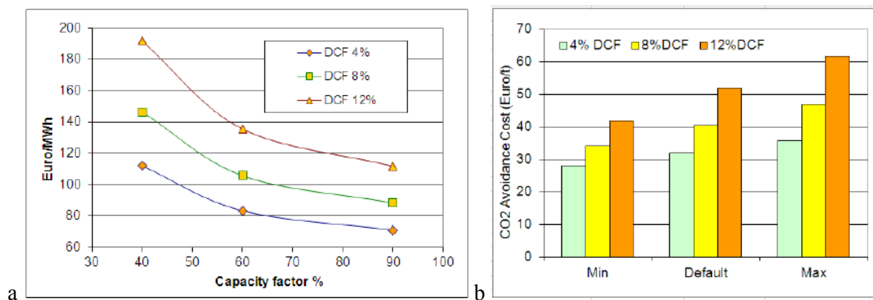
Figure 9 a) Example: sensitivity of the cost of electricity with respect to capacity factor for the cycle with oxygen membrane b) Example: sensitivity of the CO 2 avoidance cost to capital investment, for the cycle with MGD
