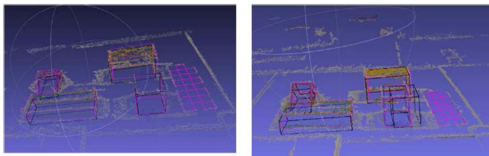
Figure 1-8: Original Fitted and Blue shift Fitted cloud
