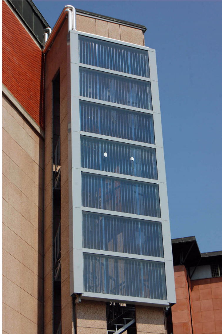
Figure 3 prototype transparent solar thermal façade collectors, installed at the pilot building in Slovenia.
