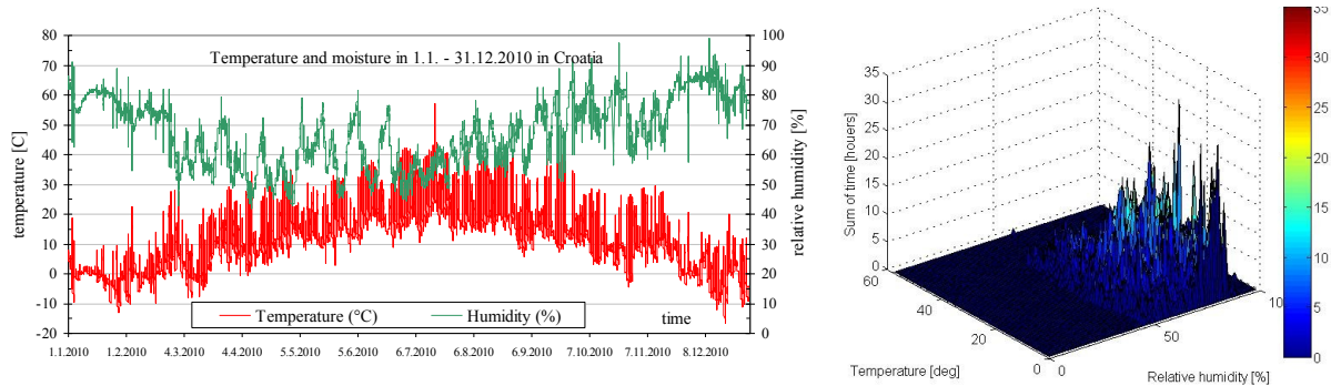
Fig. 4.2: Temperature and relative humidity was measured in four places in Europe. The graph shows the history inside a stone-wool cored sandwich panels measured in Zabok, Croatia during the year 2010. The second graph shows the sum of the measured combinations in hours in steps of 1°C and 1%.
