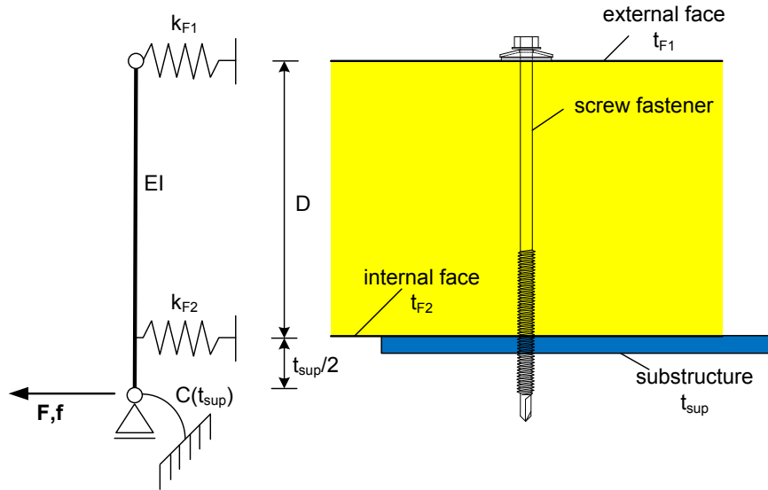
Fig. 3.4: Mechanical model of a direct fixing
