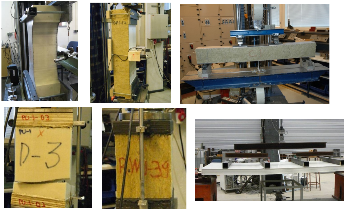
Fig. 4.1: Bone-shaped and rectangular wrinkling test specimens, shear test specimen, cross-panel tensile and compression test specimens and full-scale specimens made of PU- and ESP-foam cored and stone-wool cored sandwich panels were used in the durability studies.
