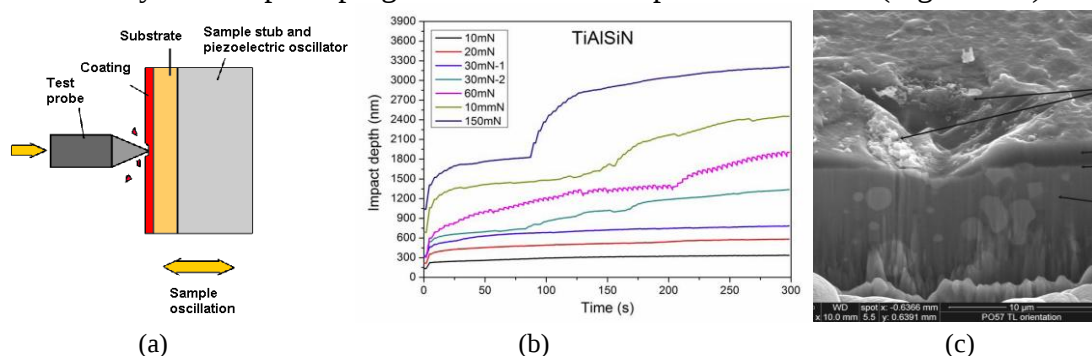
Fig. 3.4-3: Nano-impact (a), crater depth v. impact number (b) and FIB/SEM crater (c).
