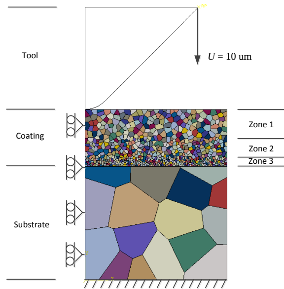
Fig. 3.5-3 Multi-zone model for CPFE simulation
