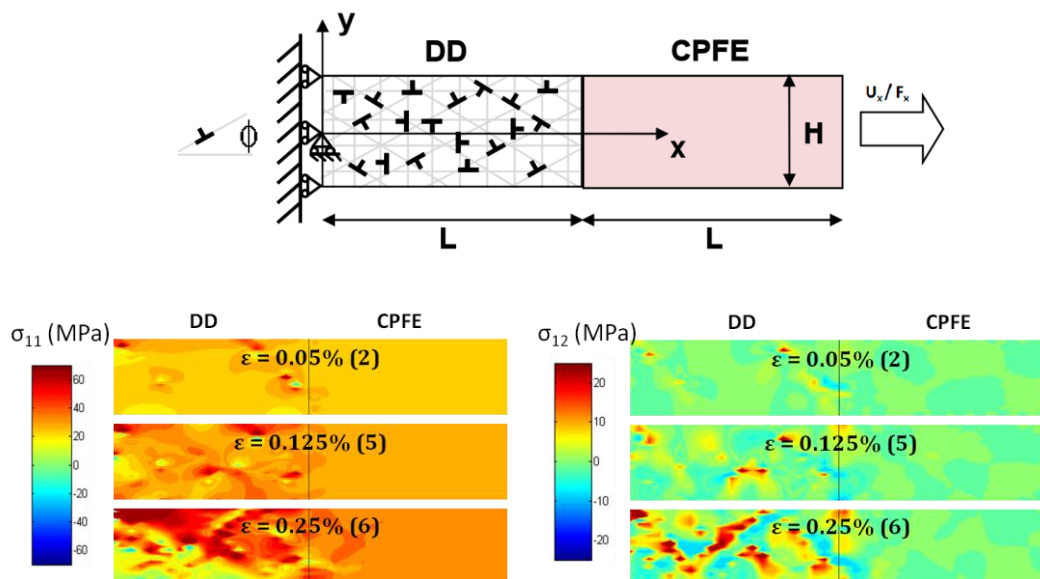
Fig. 3.5-4: Stress contours for coupled systems at step 6, \varepsilon=0.25\% .
