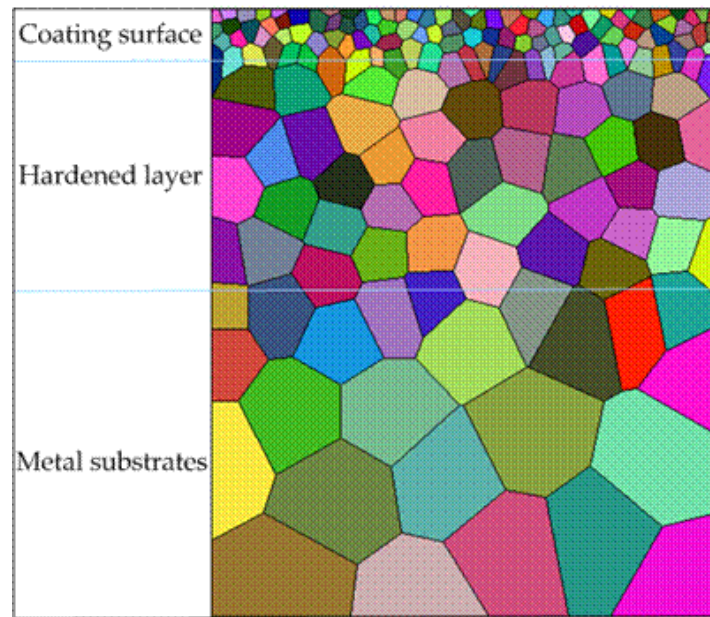
Fig. 3.2-6: Multi-zone VGRAIN model for CPFE simulation
