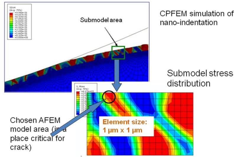
Fig.3.5-6 An example of CPFEM coupling to AFE
