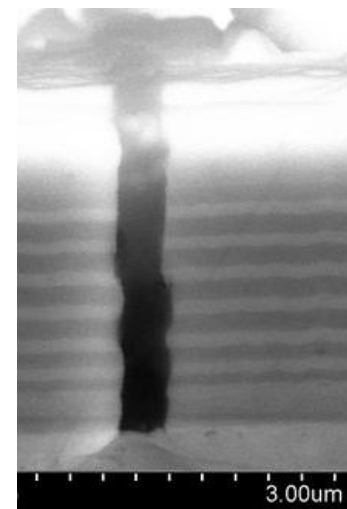
Fig.3.4-6: Zigzag cracking
