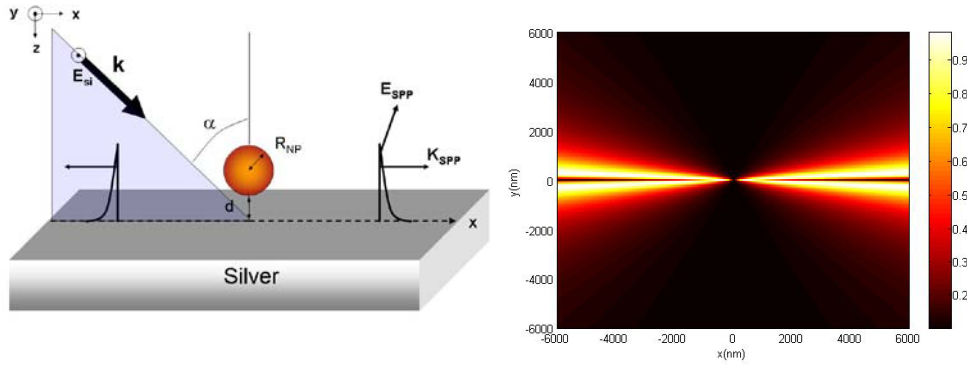
Figure 1: (Left) Scheme for the local excitation of a SPP by a MO nanoparticle (iron) on a flat metallic substrate (silver). The magnetic field is oriented along the x-axis (LMOKE configuration). The excitation wavelength is \lambda=800 nm. (Right) Top view of the modulated SPP field (modulated LMOKE signal) on the silver surface.
