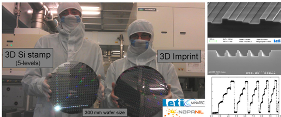
Figure 6. 300 mm Si stamp with 5-level tiered patterns and the corresponding imprinted replica..
