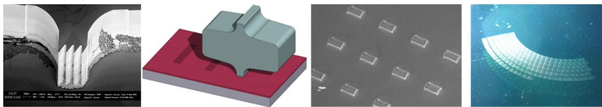
Figure 8. A single electroplated saw-tooth stamp made by X-ray lithography is used to make a larger stamp by Step&Stamp nanoimprinting. The working stamp can then be used to create rather complicated surfaces. These can be transferred to the Roll-to-Roll process for high throughput manufacturing.
