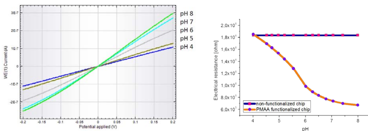
Figure 3.5 Left: Current-voltage measurement of PMAA functionalized nanoporous chip (4 x pore diameter 400 nm) at varied pH values. Right: Electrical resistance of PMAA brush functionalized nanopore chip at varied pH values. Control shows that response is not influenced by variation in pH of the phosphate buffer solution, so only by the pH-responsive polymer brush.
