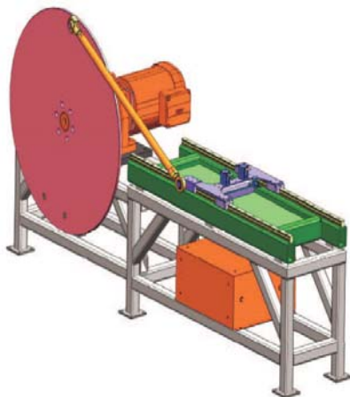
Figure 7.2b(i) The CAD model of the rig and the actual lube oil distribution test rig
