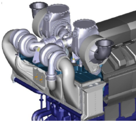
Figure 3.1a. Installation of 2-stage turbocharging system on the 4-stroke (left) and 2-stroke (right)
