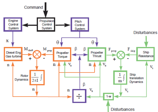
Figure 6.1a. General block diagram of ship propulsion dynamics
