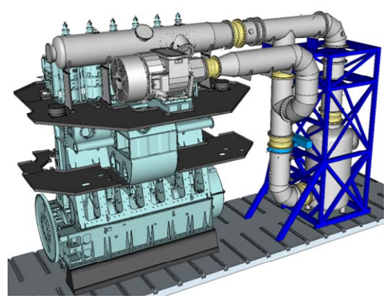
Figure 5.1b. NO x reduction technologies: CAD model of the DWI system on the RTX-4 test engine (left) and SCR system on the RTX-5 test engine (right)
