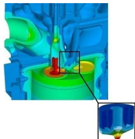
Figure 5.2b. The 4-stroke test engine with the SCR unit (left) and the temperature study on that SCR engine (right)
