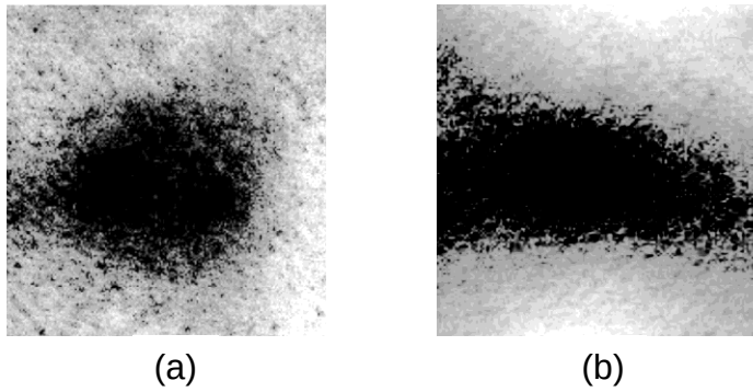
Figure 11. Processed NIR image of a 5mmx5mm delamination defect, (a); Processed NIR image of the reverse side of the same delamination.
