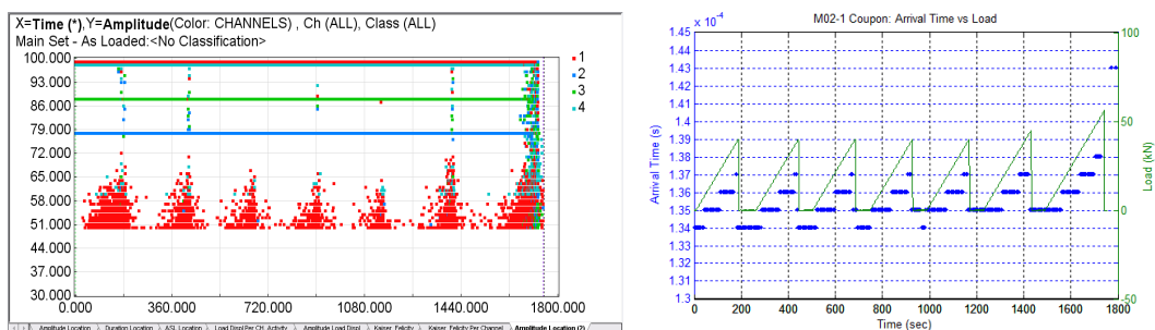
Figure 25. ComPair Monitoring system software showing detection of tensile loading cycle: AE activity to destruction, left; LRU GW activity to destruction, right
