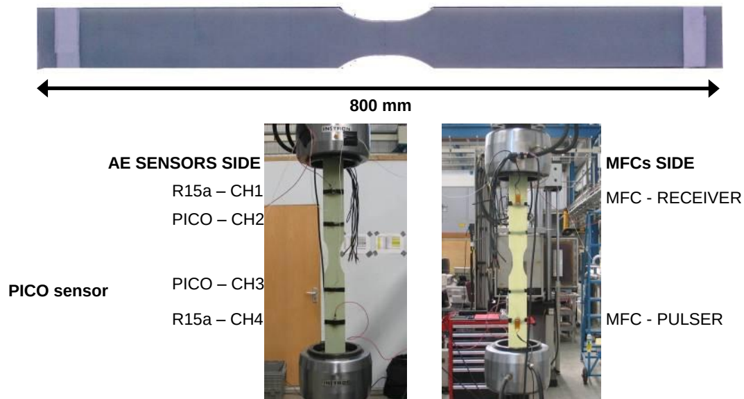
Figure 24. ComPair Monitoring AE/LRU system during a tensile test on 800mmx70mmx4mm GFRP coupon
