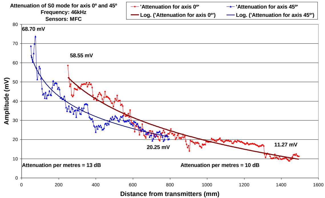
Figure 13. Attenuation characteristics of gausi-isotropic GFRP using MFC sensors as Tx and Rx
