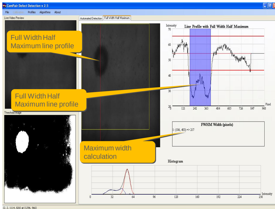
Figure 19. ComPair inspection software – Full Width Half Maximum (FWHM) implemented on impact related defect
