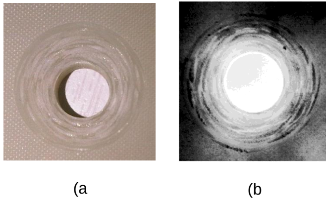
Figure 10. Close-up image of a 6.35mm countersink defect, (a); Processed NIR image of countersunk defect, (b).
