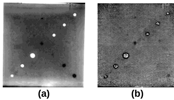
Figure 12. Results by NIR vision, (a); thermography (processed using pulsed phase thermography), (b)
