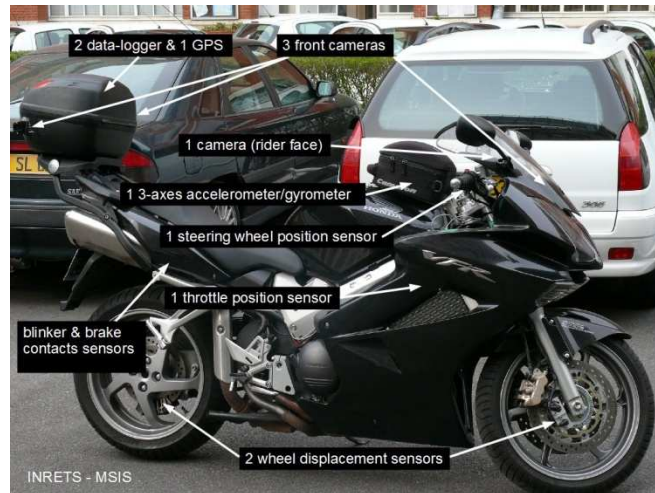
Figure 1: Example of instrumented motorbike for pilot naturalistic study
