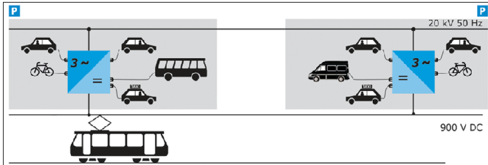
Figure 5 – Opportunity of using DC traction systems for charging battery-powered vehicles
