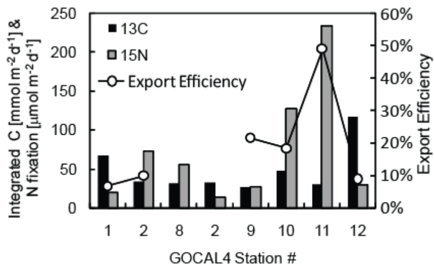
Figure 1. Integrated C production and N 2 fixation rates. Integration depths varied from the upper 45m at Stations 1-9 and the upper 60m at Stations 10-12. Estimates of carbon export efficiency, derived by comparison of sediment trap and 234 Th derived POC fluxes with integrated C production rates are also shown.
