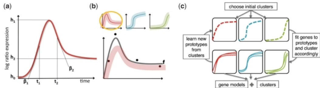
Figure.: An integrative clustering-modeling algorithm. (A) The impulse model capturing a two-phase temporal response by a product of two sigmoids, with parameters: onset time ( t_1 ), offset time ( t_2 ), the original baseline height ( h_0 ), peak response height ( h_1 ), new baseline height ( h_2 ), onset rate ( \beta_1 ) and offset rate ( \beta_2 ). (B) Fitting the model to the data with mixture priors on the parameters (bottom), which are distinct prototypes of responses (top). (C) A scheme describing our integrative clustering and modeling algorithm DynaMiteC: (i) Choosing initial clusters. (ii) Iterating between optimizing the fit to the genes and optimizing the prototypes. (iii) The resulting models per gene and clusters.
