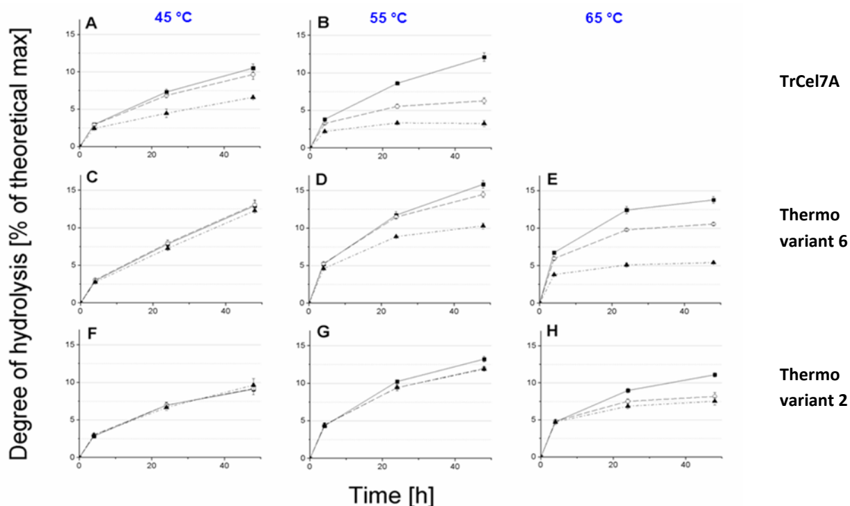
Figure 3: Hydrolysis of Avicel (10 mg/ml) in the presence of lignin by the two novel GH7 Thermo enzyme variants and T.reesei Cel7A, a reference. Hydrolysis was performed at three different temperatures (45, 55, and 65 °C) at pH 5 with and without added lignin. Reactions without added lignin (■), with 10 mg/ml of wheat straw EnzHR lignin added (○) and with 10 mg/ml of spruce EnzHR lignin added (▲). Hydrolysis reactions were supplemented with 500 nkat/g cellulose with a thermostable \beta -glucosidase (Roal), and assays performed in triplicates. Solubilized reducing sugars were measured with the PAHBAH reagent. Results are presented as percentage of the theoretical maximum glucose yield from 10 mg/ml of Avicel.
