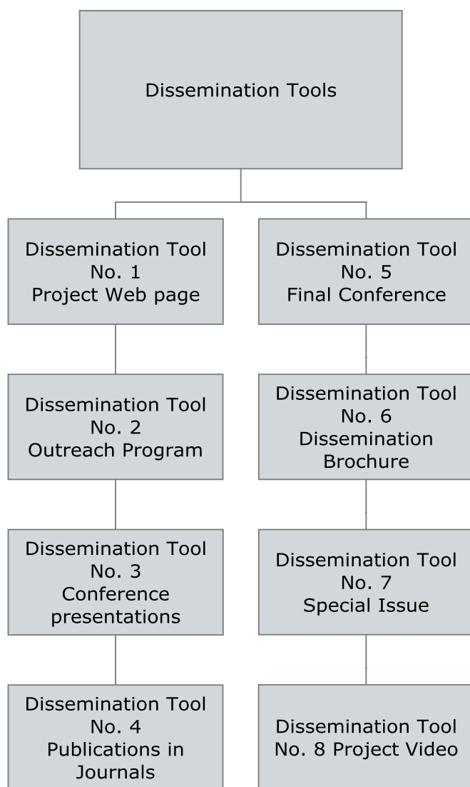
Figure 1: Dissemination Tools
