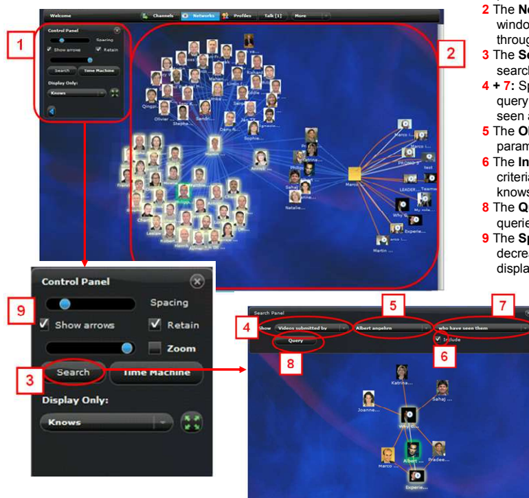
Figure 8: Operating the Networks Visualization Pane in CRISISTUBE
