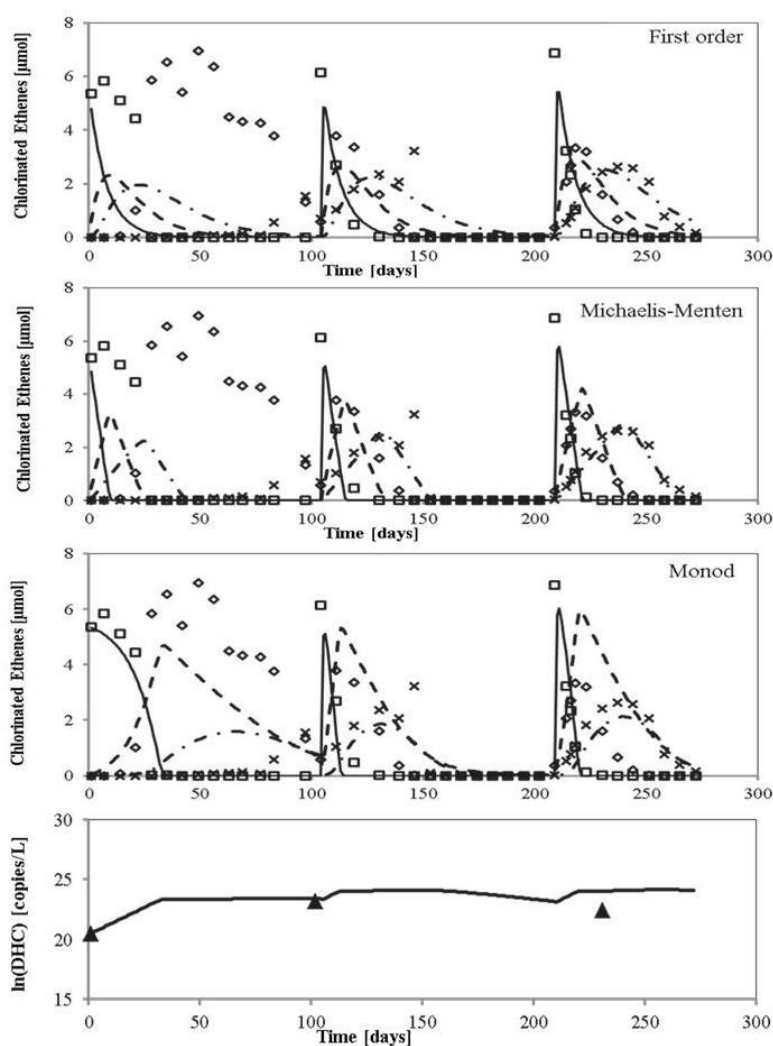
Figure 14: Model results using First-order (top), Michaelis-Menten (middle) and Monod (bottom) kinetics for the aquifer of one location to which sediment extract was added. Observed data: \square TCE, \diamond cDCE, \times VC and \blacktriangle 16S rRNA gene copy numbers of Dehalococcoides mccartyi . (DHC). Modeled data: — TCE, ---- cDCE, -.- VC and — cell numbers of DHC. The 16S rRNA copy numbers were calculated from triplicate qPCR measurements and are presumed to represent DHC cell numbers in a 1 to 1 relationship.
