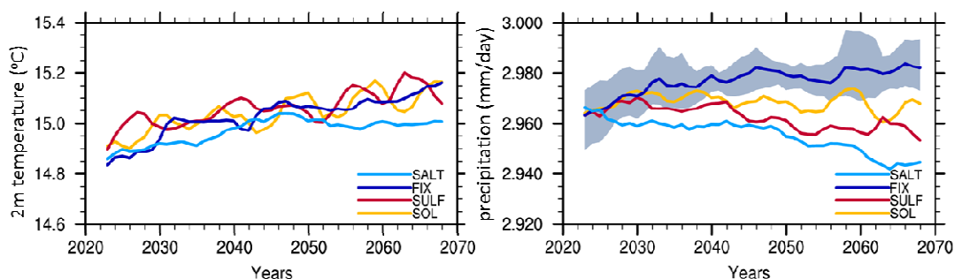
Figure 9: Time evolution of global mean temperature (°C, left) and precipitation (mm/day, right) simulated with the MPI-ESM under four different scenarios of type G3, i.e. where it is attempted to keep the climate forcing constant at 2020 levels through different methods. SALT: manipulation of marine clouds; FIX: GHG concentrations fixed at 2020 levels; SULF: injection of sulfur into the stratosphere, SOL: reduction of solar irradiance. All results are 5-year running means averaged over ensemble simulations with three members. The shading around the precipitation time series from FIX indicates maxima and minima of the ensemble members.
