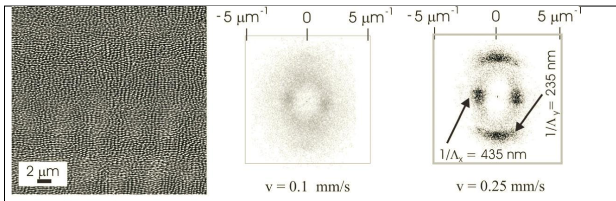
Figure 1. SEM photograph of silicon processed in methanol (left), and 2D fast Fourier analysis of silicon processed at a rate of 0.1 mm/s (centre) and 0.25 mm/s (right)
