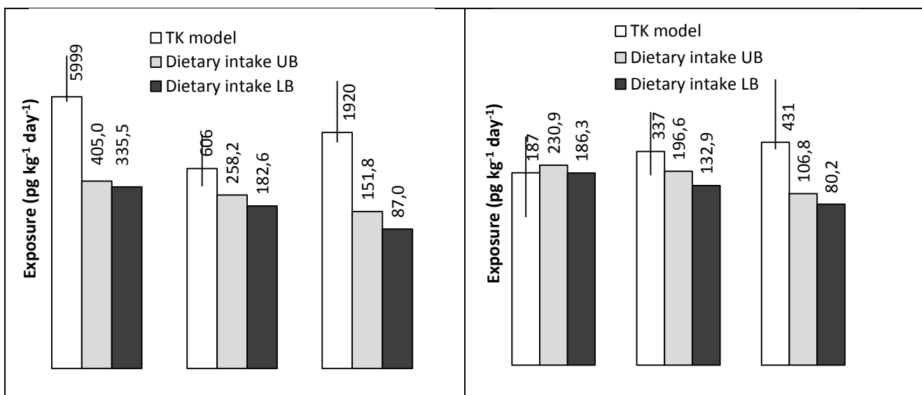
Figure 2.6.2. Comparison of reconstructed total exposures (TK model) and estimated average dietary intakes of PFOS (left) and PFOA (right) for the Belgian (BE), Italian (IT) and Norwegian (NO) population. Solid white bars represent reconstructed intermediate (median) exposure and the error bars depict the low and high exposure. Light grey and dark grey solid bars represent the upper bound (UB) and lower bound (LB) assumption for non-detects respectively.
