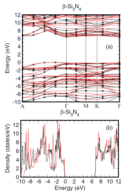
Figure 2: (a) Band structure and (b) electronic density of states of \beta -Si 3 N 4 . The sc-QPGW results are shown as black lines, while the MBJLDA results are represented by red lines.
