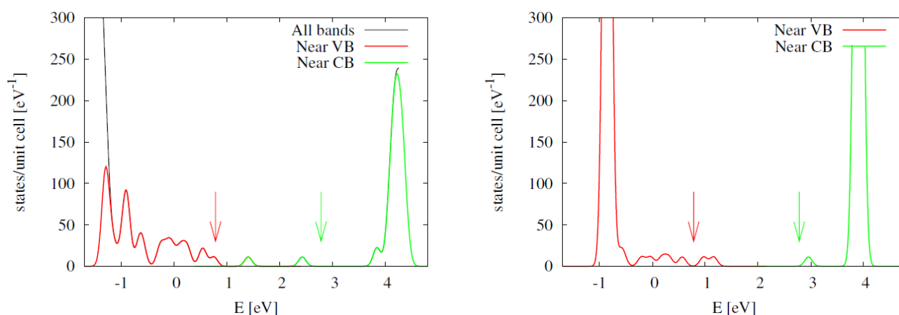
Figure 3: Density of states (DOS) for the 1k- and 100k-Si 3 N 4 system (left and right panels, respectively). For the 1k system, the black line is the result from a standard DFT calculation. The colored lines are obtained using the harmonic Davidson inner eigenvalue solver, and were determined in two separate runs, with reference energies \epsilon_{ref} at the positions indicated by the arrows. The zero of the energy axis is set to the Fermi energy.
