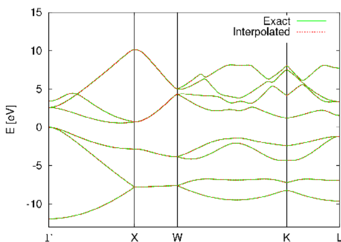
Figure 5: Band structure for silicon using an exact calculation (charge density taken from a 24 \times 24 \times 24 k-mesh) and an interpolation from a 6 \times 6 \times 6 k-mesh. The energy differences are in the meV range.
