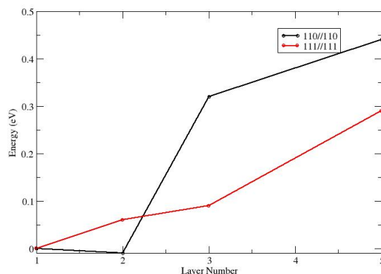
Figure 14: Energies of P doping of Si at the Si/Ag interface. In both cases energies are offset to the energy of layer 1. The layers are listed in ascending order moving away from the interface.
