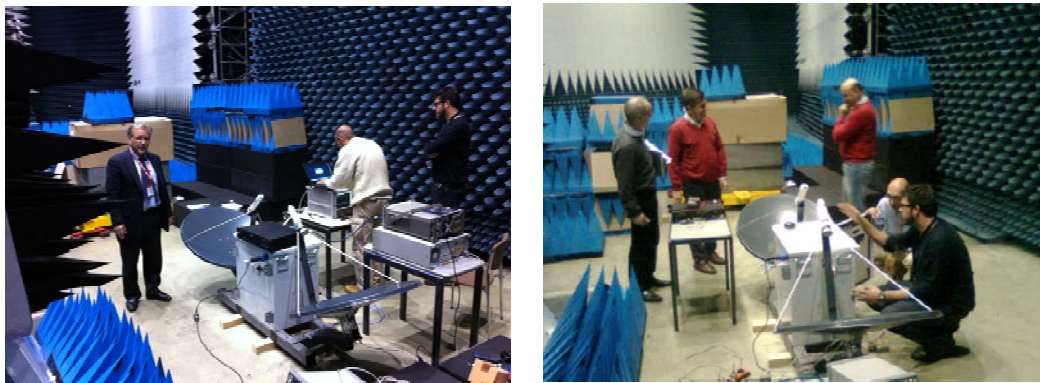
Figure 8. The prototype microwave built in this Project at the Compact Payload Test Range facilities in the European Space Agency, Noordwijk, the Netherlands in 2012.
