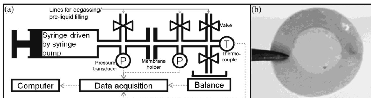
Figure 1. (a) Schematic of the setup built to perform fluid flow measurements in hydrophilic alumina nanoporous membranes, one of which is shown in (b). 2
