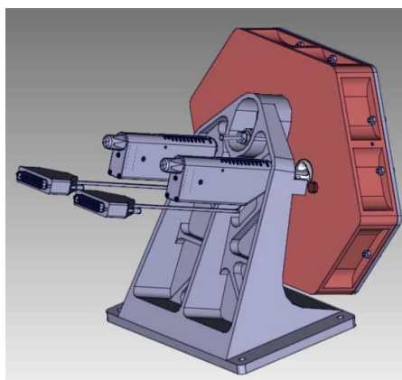
Figure 22 Overall view of the 50°moving mirror
