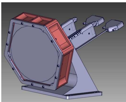
Figure 22 Overall view of the 50°moving mirror
