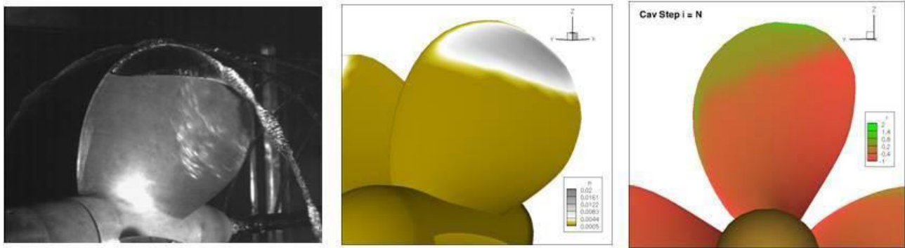
Figure 23: Cavitating flow modelling by BEM
