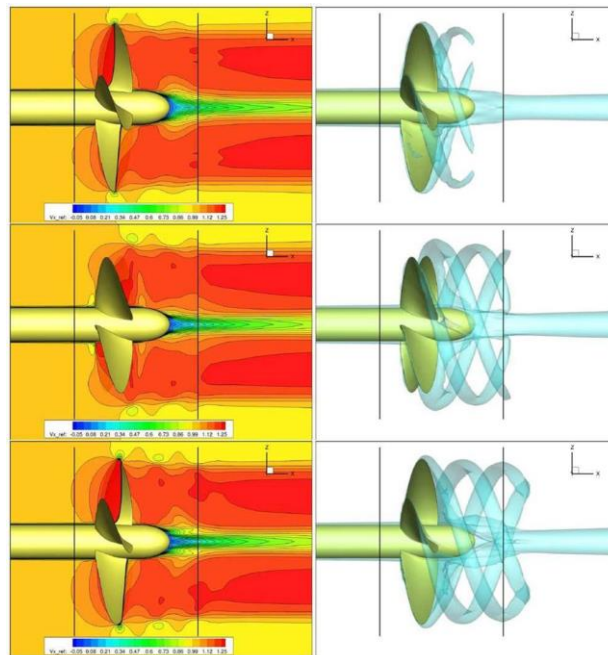
Figure 20: Propeller results using sliding interfaces (from top to bottom) Coarse, medium, fine grid
