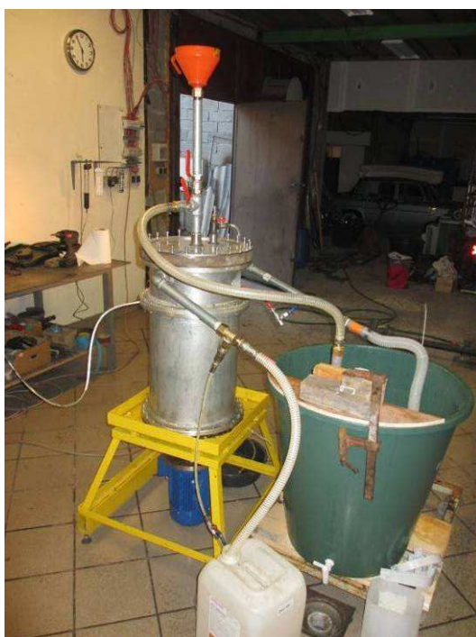
Figure 5: Experimental configuration for optimization tests in Ruffieux.
