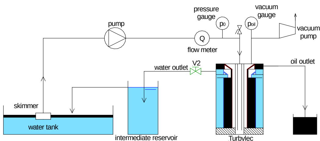
Figure 7: Flow loop for experimental characterisation of skimmer + pump + TURBYLEC system.
