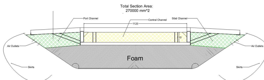
Figure 2: The soft hull made of Polyethylene connected to the rigid structure
