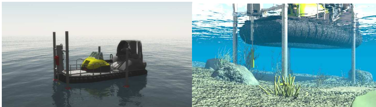
Figure 19: Hovercraft set up for geophysical surveys
