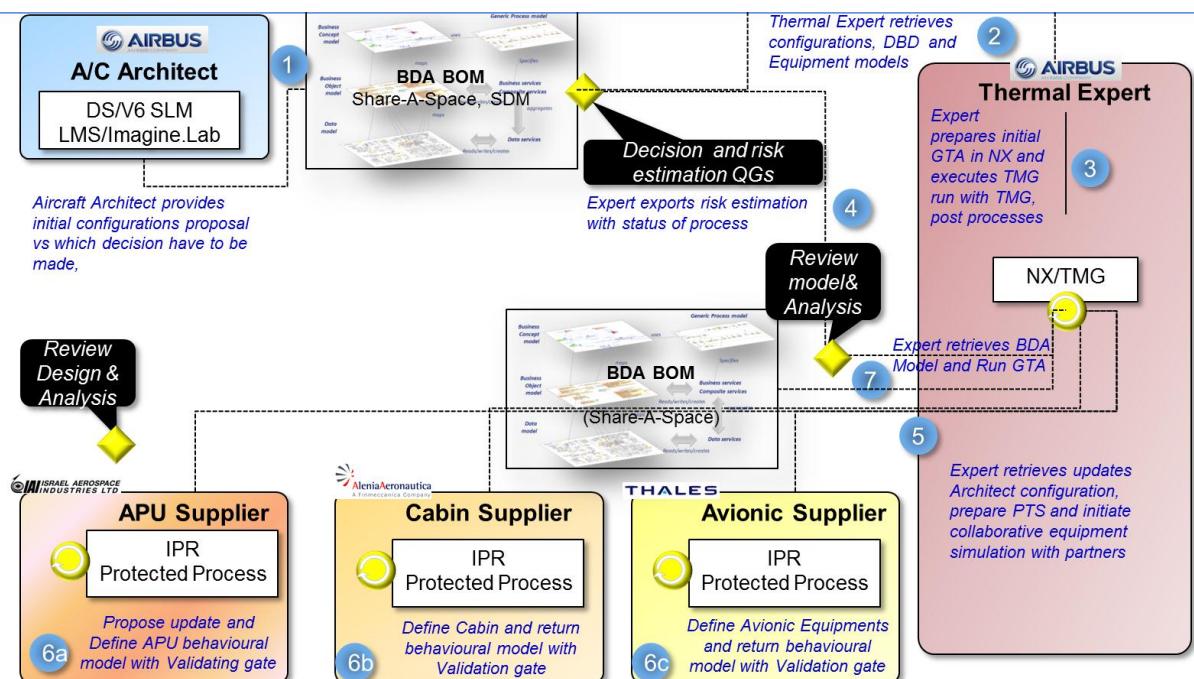
Figure 44: Developing the Thermal Aircraft along the lifecycle
