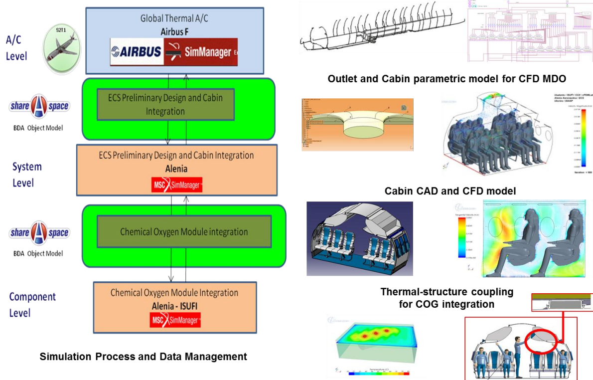
Figure 48: Cabin systems preliminary design integration and optimisation for passenger comfort
