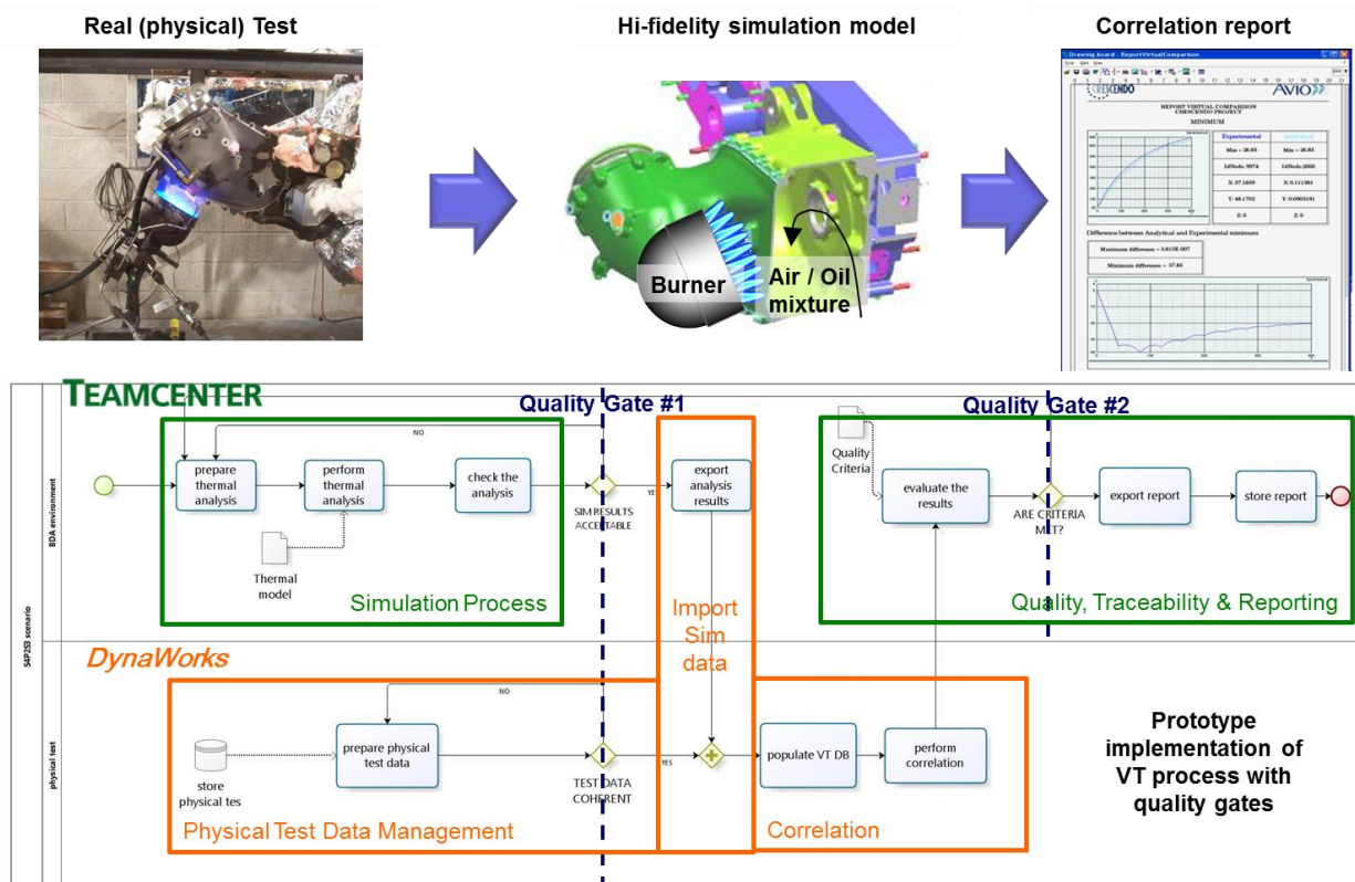
Figure 62: Virtual Testing process for engine fire protection certification
