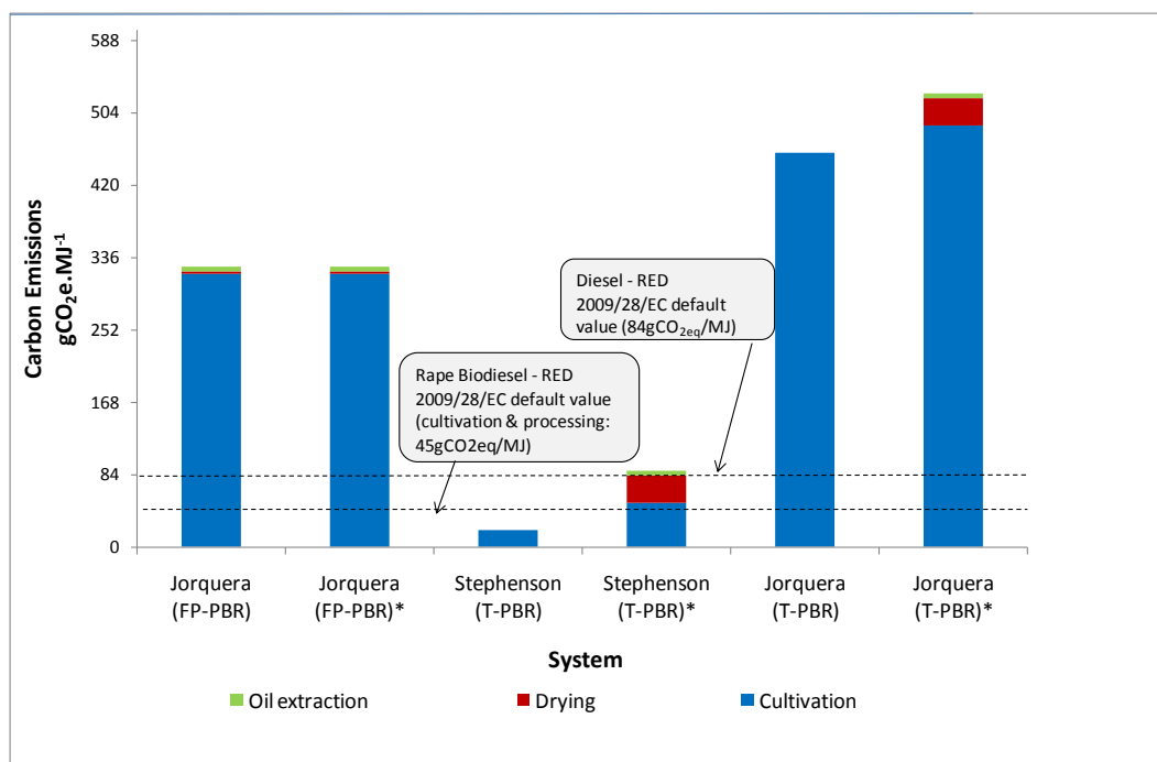
Figure 14: Illustrative estimates for CO 2 emissions from photobioreactors
