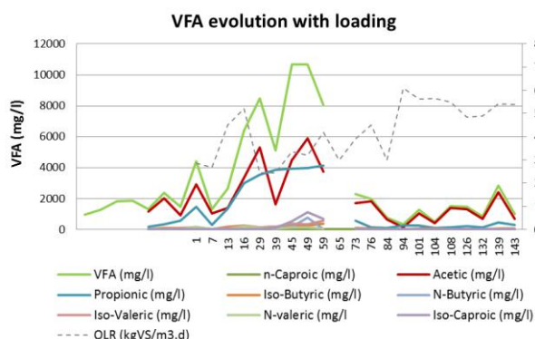
Reduction in VFA after adding Se and Co on day 51
