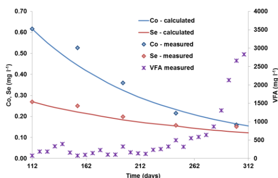
Dilute-out curve used to estimate critical concentrations of Se and Co
