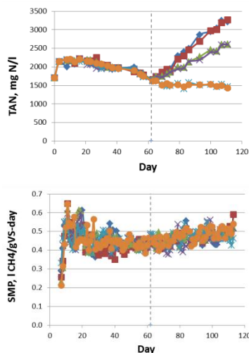
TAN and specific \text{CH}_4 production in digesters at no, 1:1 and 1:2 dilution
