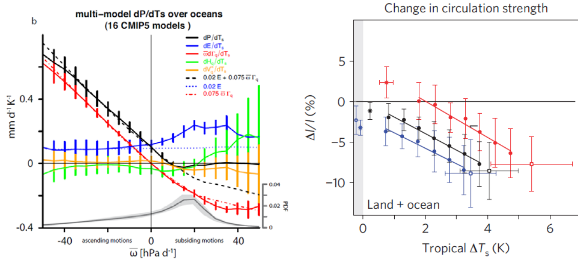
Figure 12 left: Sensitivity of precipitation, and of its different components, to sea surface temperature changes estimated through linear regression from abrupt4xCO2 simulations. Right: Response of the tropical atmospheric circulation to increased CO2 in a range of CMIP5 experiments. For land (red) and ocean (blue) areas, evolution with surface warming of the multi-model mean fractional change (compared with pre-industrial) in the strength of the overturning circulation. (From Bony et al. 2013 Nature Geoscience)
