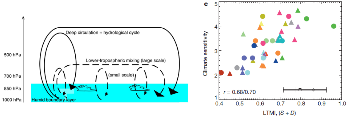
Figure 10: Left: Deep overturning strongly coupled to the hydrological cycle and atmospheric energy budget is shown by solid lines; lower-tropospheric mixing is shown by dashed lines. Right: Relation between the intensity of low tropospheric mixing (LTMI) and the climate model sensitivity for a number of climate models (from Sherwood et al 2014)
