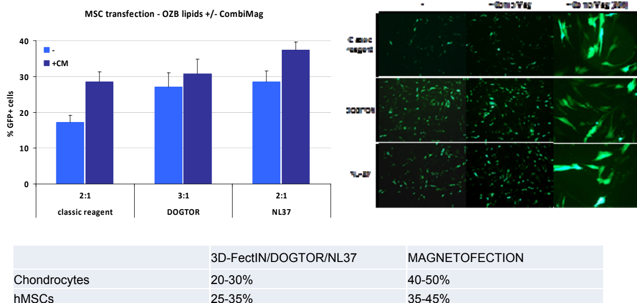
Fig. 1.4: Selection of the best formulation to transfect chondrocytes and hMSC in classical cell culture conditions. DOGTOR and NL-37 induced higher transfection efficiency in terms of number of cells transfected and transgene expression. Moreover, Magnetofection (CombiMag) allowed raising the transfection efficiency of both reagents.
