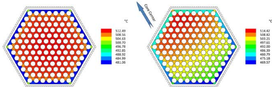
Figure 10. Coolant outlet temperature distribution among the sub-channels of the most powerful FAs: on the left the central one; on the right the one in the outer core region.
