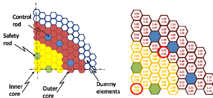
Figure 9. Final ALFRED core configuration (left) and BoC (upper value) and EoC (lower value) power (in MW) per FA distribution (right).
