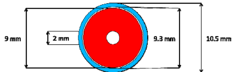
Figure 8. ALFRED fuel pin cross-section.
