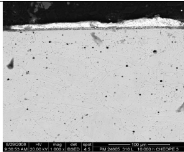
Fig 20a) 316L after exposure in Pb (10-6wt% oxygen) at 550°C for 10,000h
