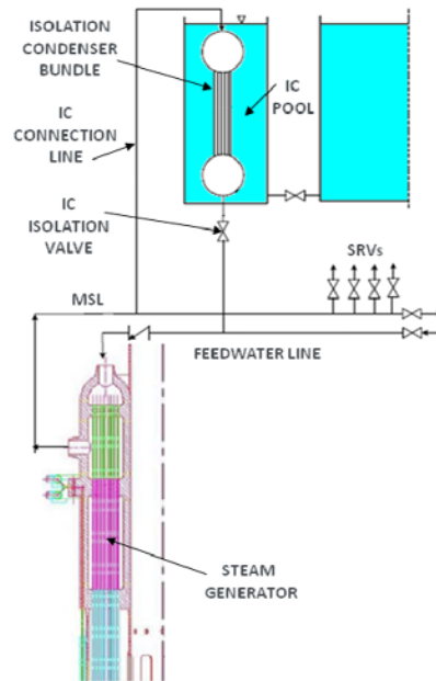
Figure 7: Isolation condenser
